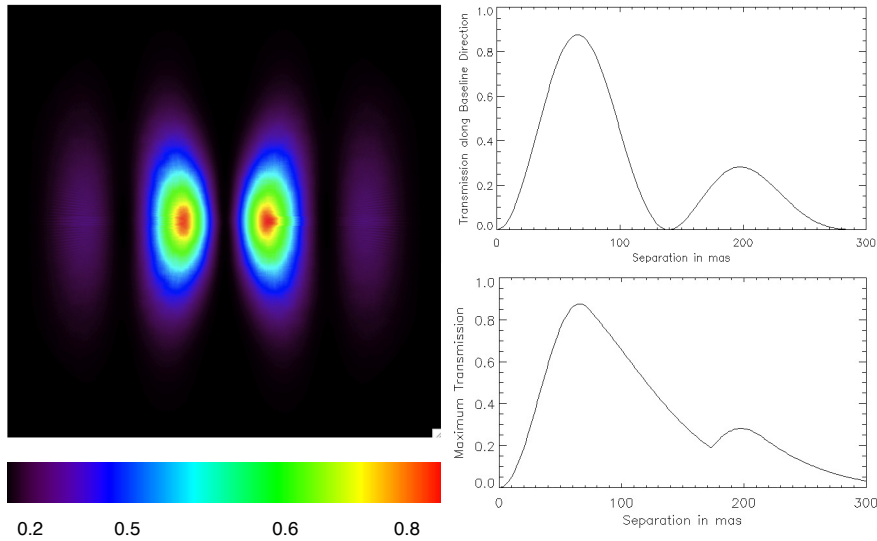
FIG. 1.— Left: PFN sky transmission over 0.6'' \times 0.6'' field of view, assuming a "horizontal" 3.20 m baseline separating two elliptical sub-apertures (3 m \times 1.5 m). Top right: PFN transmission vs separation, along baseline direction. Bottom right: Maximum transmission versus baseline rotation angle, as a function of separation.
