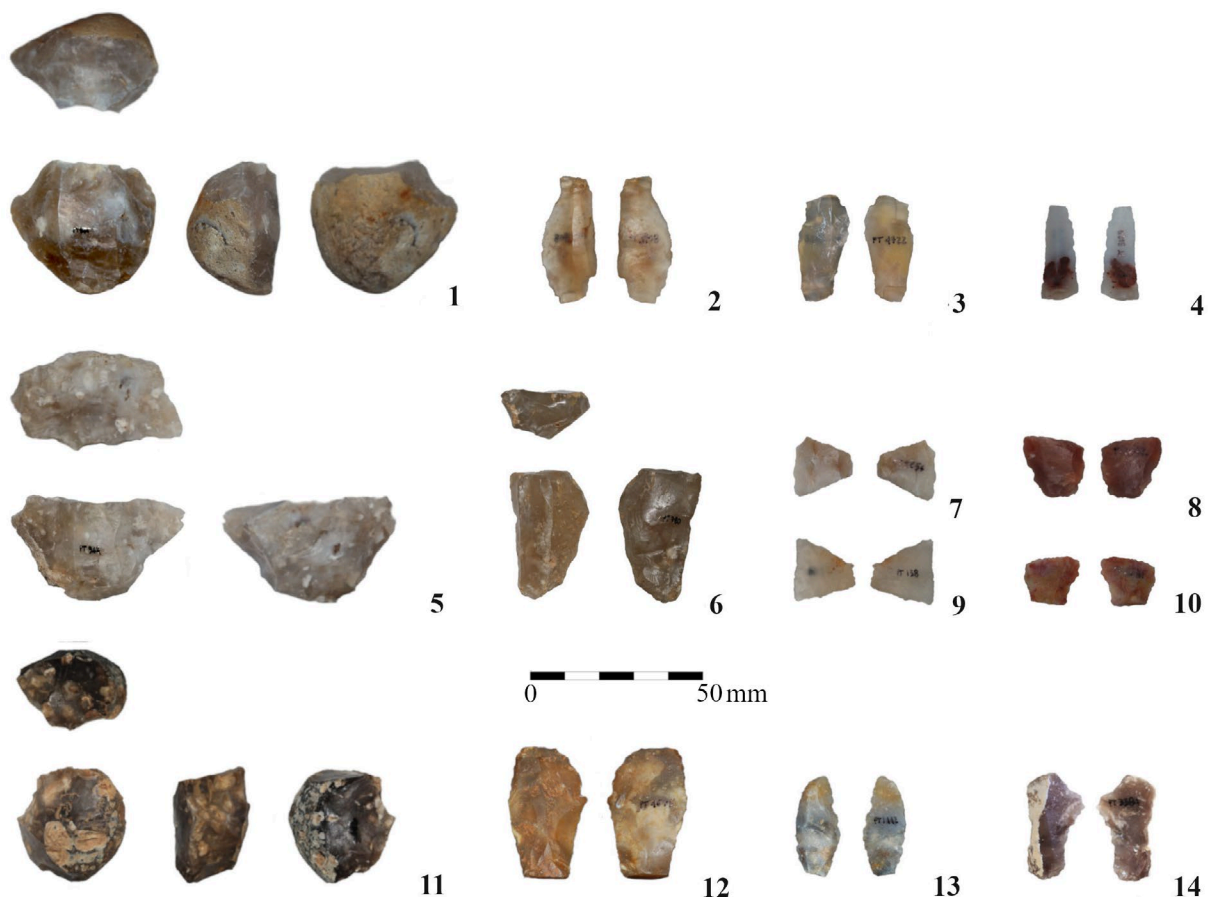
Figure 6. Chert lithic assemblage from the EN site of Su Paris de Sa Turre, Santa Caterina di Pittinuri, Cuglieri (OR) (mid of the 6 th millennium BCE). Bladelet core (1, 5) and bladelet core side (6) with a single striking platform; flake core with multiple striking platforms (11); blade(let)s (2-4) and flakes like bladelet (12-14); truncations (8, 10) and geometrics (7, 9) (photograph by B. Melosu).
