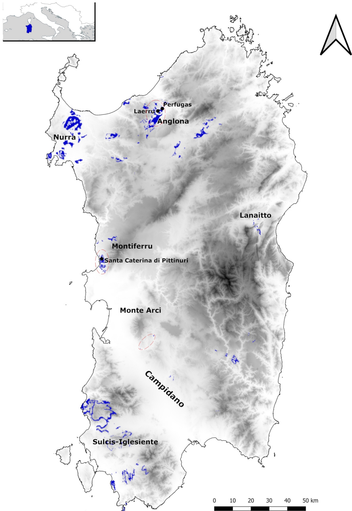
Figure 1. Sardinia chert bearing formations ( data source available online ). In red, surveyed areas.
