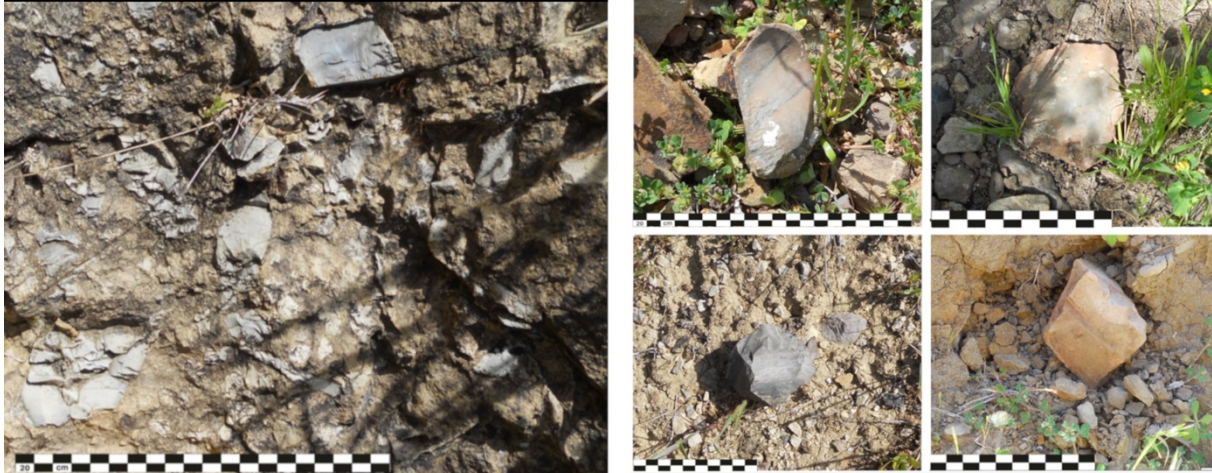
Figure 4. Chert nodules in primary position (left); chert blocks in secondary position at Rio Laccus region, Morgongiori (right) (photograph by B. Melosu).
