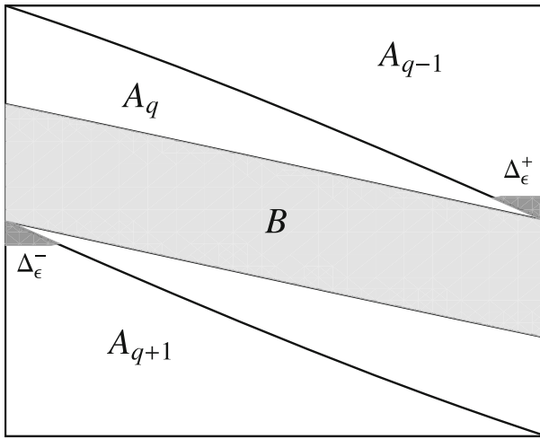
Fig. 5. The set \Delta_\epsilon
