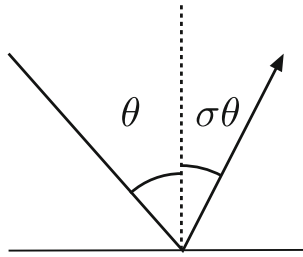
Fig. 2. Contracting reflection law
