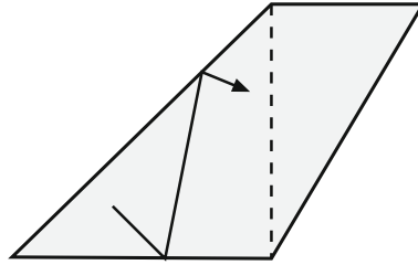
Fig. 3. A billiard with parallel sides which is uniformly hyperbolic
