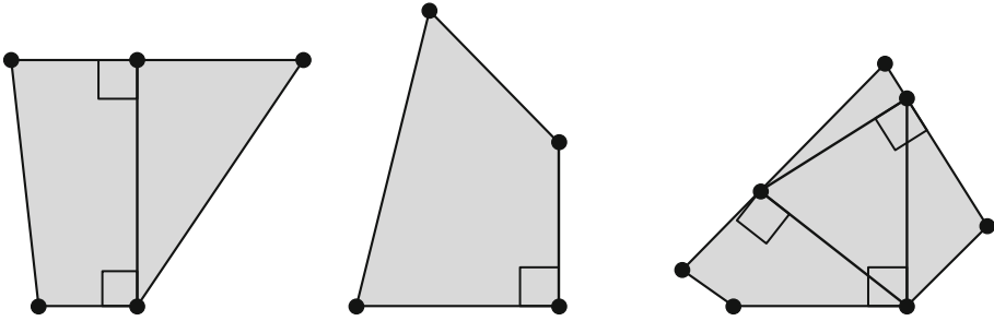
Fig. 4. Examples of polygons with orthogonal vertex connections.
