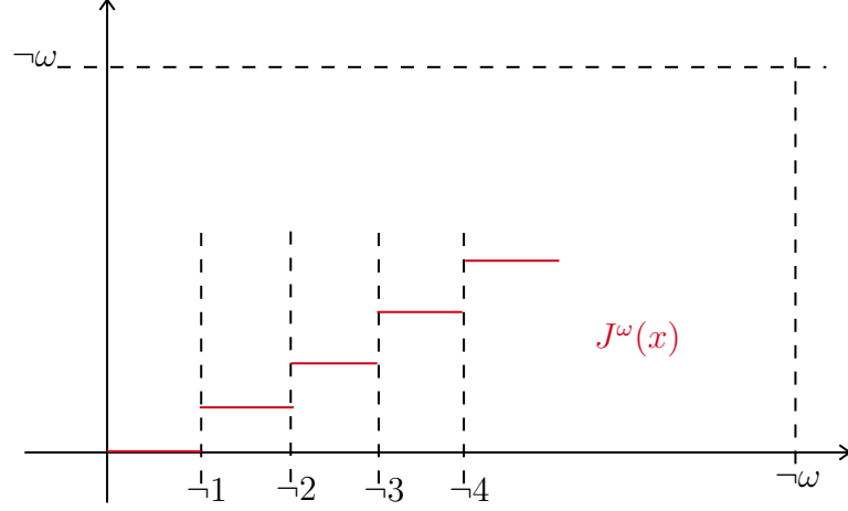
Figure 4.7: The \omega -jumping function, J^\omega
