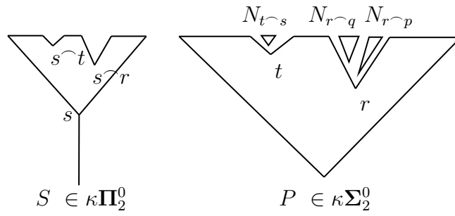
Figure 6.2: \kappa \Sigma_2^0 and \kappa \Pi_2^0 sets of \kappa^\kappa
