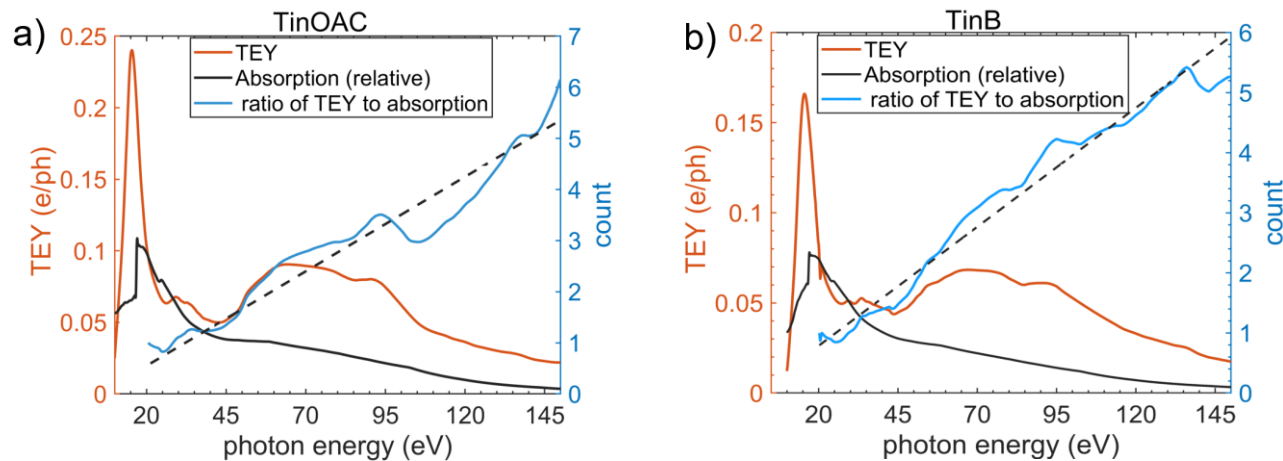
Figure 5.16. TEY (red) and absorption spectra (black) set to a same value at 20 eV, and their ratio (blue) for a) TinOAc, b) TinB. The dashed lines are linear fits to the ratios.
