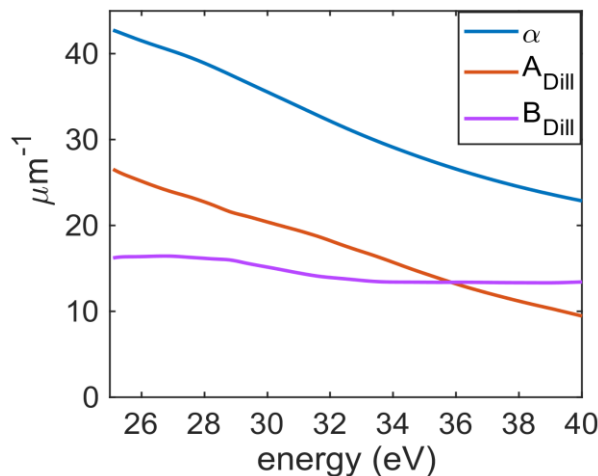
Figure 3.6. Dill parameters and linear absorption coefficient for TinOH in the XUV range.
