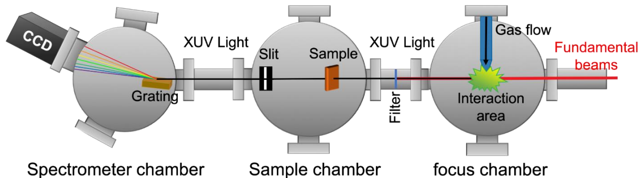
Figure 3.2. Schematic of the HHG set-up used for XUV generation. The red line shows the beam path of the fundamental beams, and the black path highlights the beam path of the generated XUV pulses.
