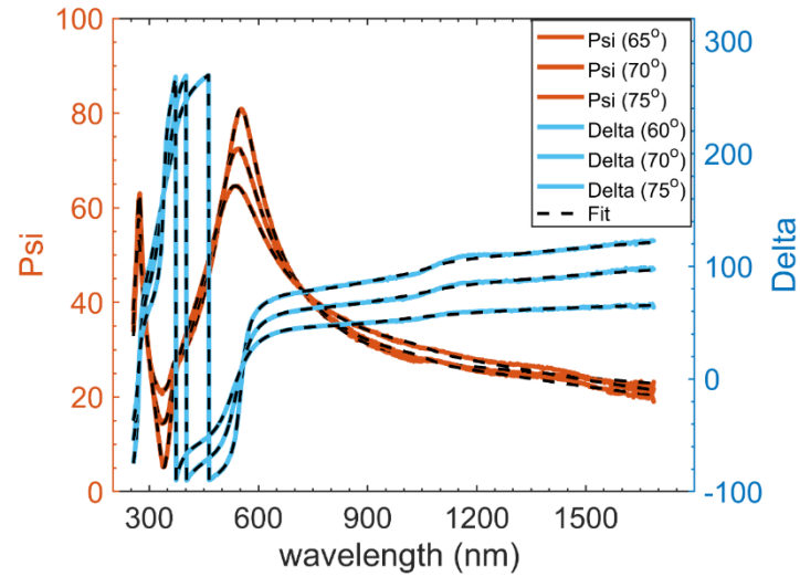
Figure 2.24. The ellipsometry data measured at three different incident angles and the corresponding fit for TinOH resist on the Si frame of the membrane using the Cauchy parameters in Figure 2.21. The measured thickness for TinOH on the frame at this spot is 78 nm.
