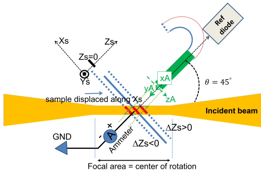
Figure 2.11. The relative positions of sample (S), electron analyzer (A), reference (Ref) diode and the incident beam in the BEAR beamline. For TEY measurements, the ammeter measures the drain current from the sample. The electron analyzer measures the intensity or and the kinetic energy of the photoelectrons in electron kinetic energy analyzer mode as in the case of XPS measurement.
