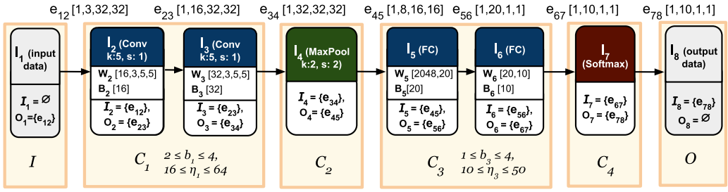
Fig. 4. An example of cluster design from a given baseline CNN. Layers of the same type are grouped into a cluster. The cluster is further made flexible to allow more layers and neurons per layer which are then constrained by definite bounds.
