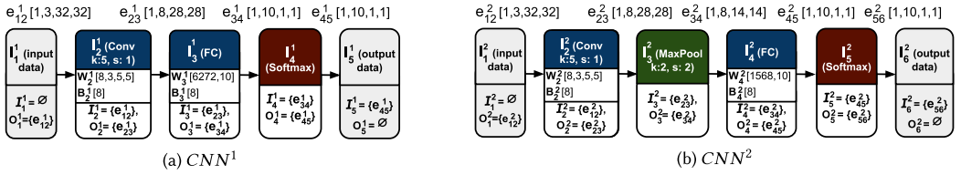
Fig. 1. CNN computational model.
