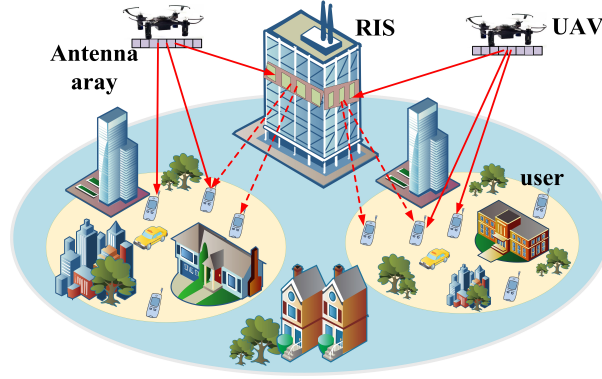
Fig. 1: Illustration of a RIS-assisted multi-UAV system with NOMA.
