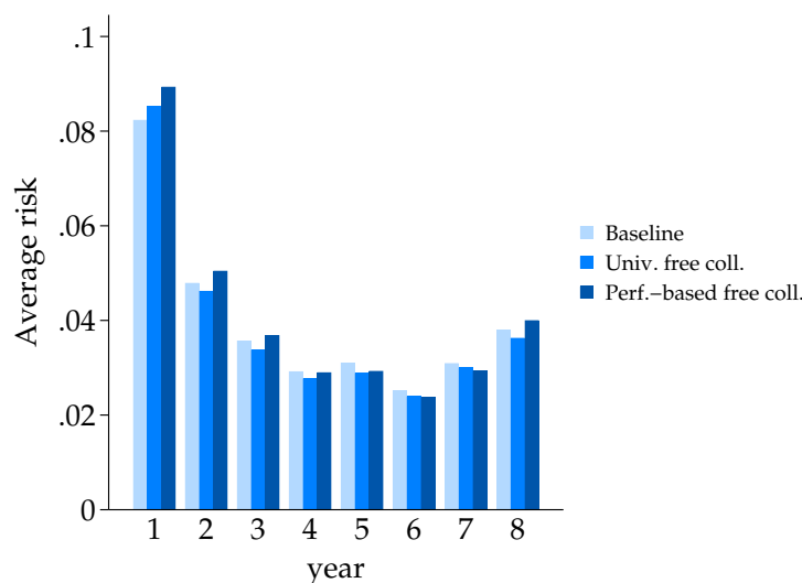
Figure 13: Anticipated Risk.
