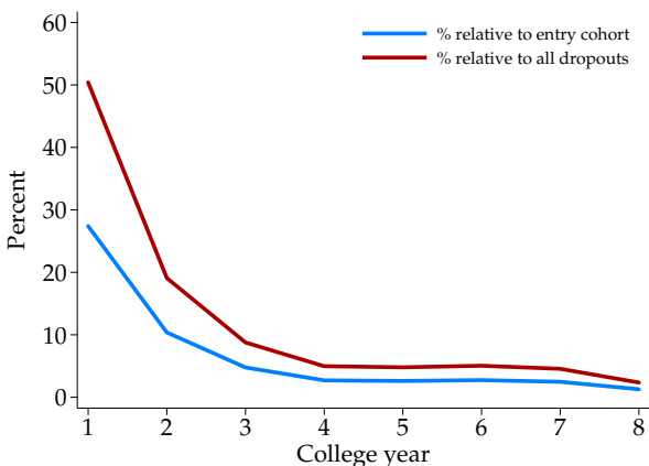
Figure 2: Dropout Timing.
