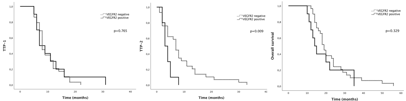
Figure 2. Kaplan–Meier analysis of survival curves according to VEGFR2 expression.
