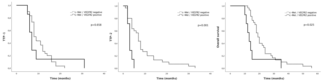
Figure 3. Kaplan–Meier analysis of survival curves according to concomitant c-Met/VEGFR2 expression.
