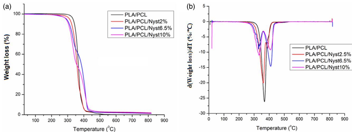
FIGURE 4 (a) TGA thermograms and (b) DTG curves of PLA/PCL/Nyst composites. [Color figure can be viewed at wileyonlinelibrary.com ]
