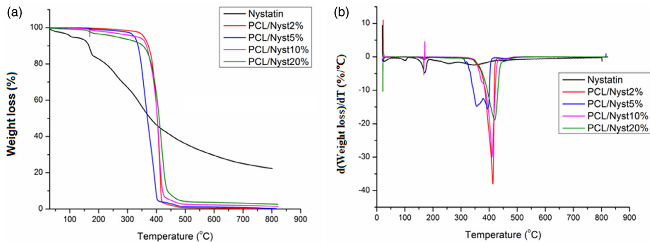
FIGURE 3 (a) TGA thermograms and (b) DTG curves of PCL/Nyst composites. [Color figure can be viewed at wileyonlinelibrary.com ]
