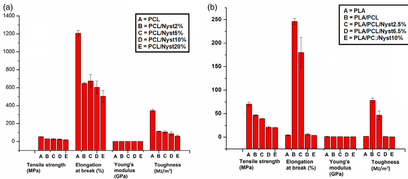
FIGURE 6 Comparison of mechanical properties of (a) PCL/Nyst (b) PLA/PCL/Nyst composites. [Color figure can be viewed at wileyonlinelibrary.com ]
