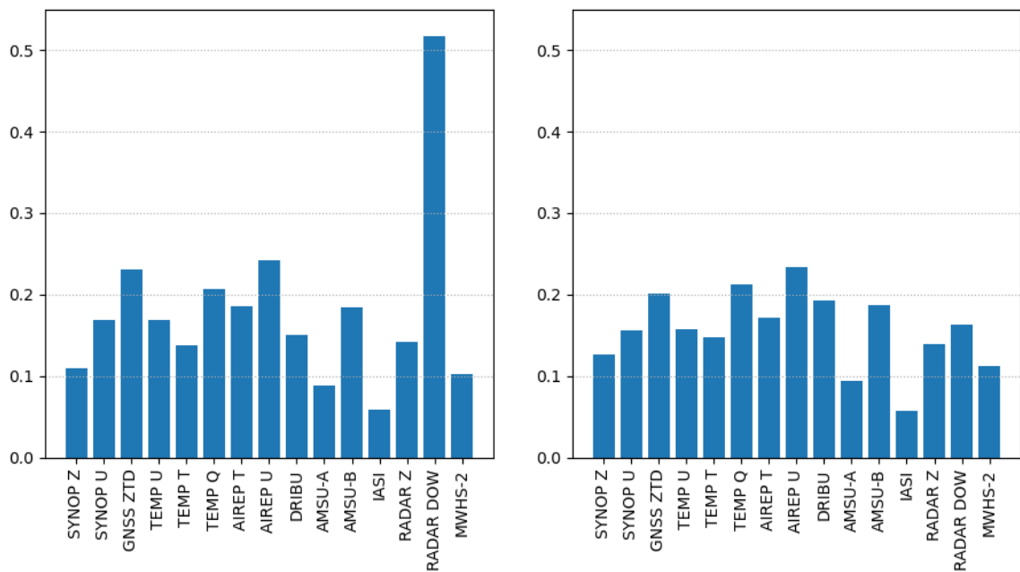
Figure 4. Relative DFS for a case with low observation error for radar radial velocity (RADAR DOW) in the left panel and for a case with adjusted, more suitable, observation error for radar radial velocity in the right panel.
