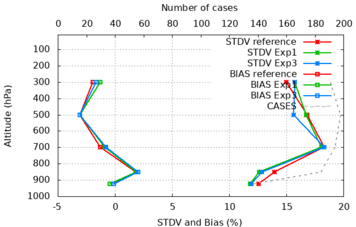
Figure 15. Verification of vertical profiles of relative humidity for the reference run (red), Exp1 (green) and Exp3 (blue). Squares (to the left) show the bias while the stars (to the right) show the standard deviation. Number of cases refers to the number of radiosondes in the verification.
