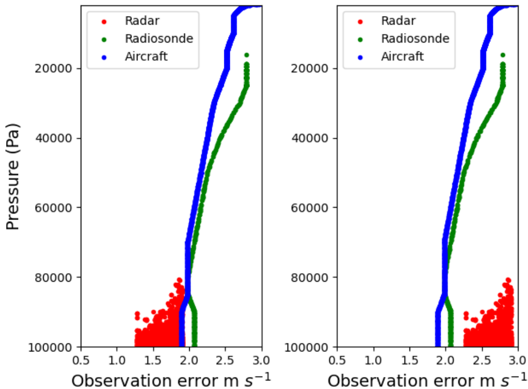
Figure 3. Value of the observation error for radar radial velocity (Radar, red), aircraft wind (blue) and radiosonde wind (green) before (left) and after (right) increasing the observation error for the radar radial velocity.
