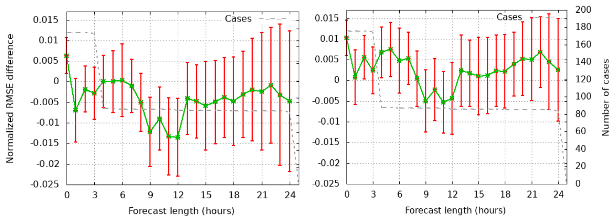
Figure 8. Significance test of normalized RMSE for mean sea level pressure for Exp1 compared to the reference experiment (left) and for Exp3 compared to the reference experiment (right). Positive values means smaller RMSE for the wind experiments and thus a positive impact on the forecasts. The number of cases refers to the number of verification times.
