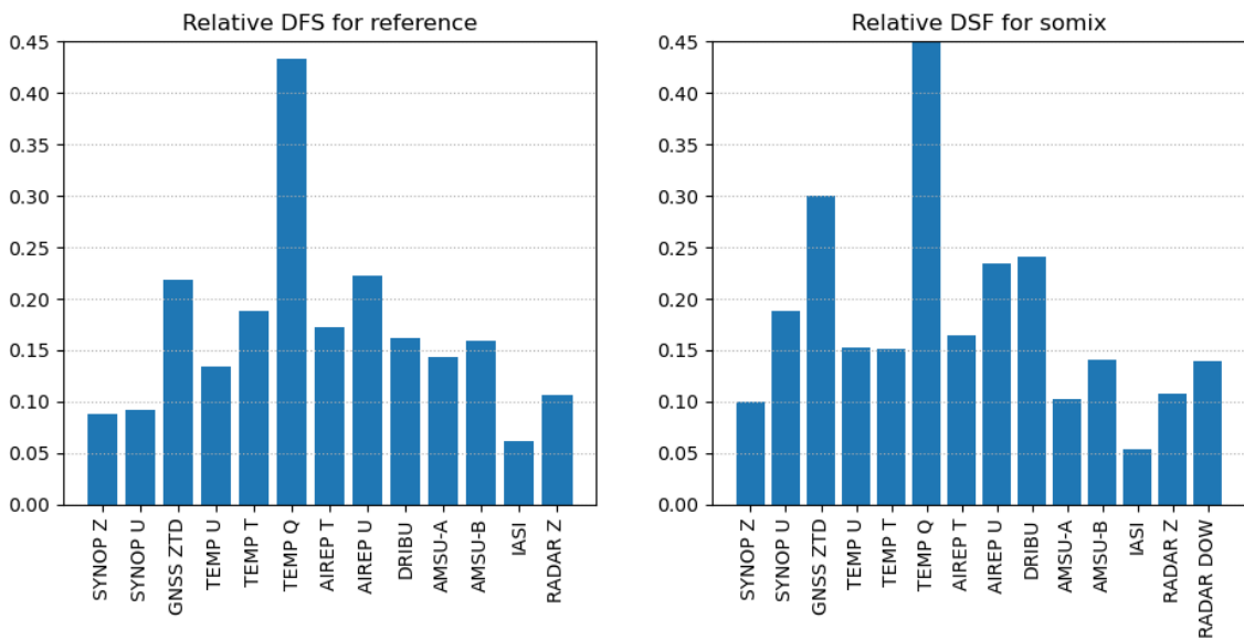
Figure 17. Same as Figure 16 but during a situation with stratiform precipitation, 20210817 at 18.00 UTC.
