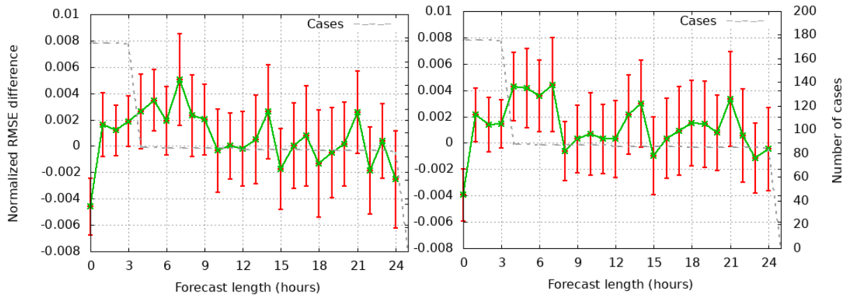
Figure 6. Significance test of normalized RMSE for wind speed at 10 meters for Exp1 compared to the reference experiment (left) and for Exp3 compared to the reference experiment (right). Positive values means smaller RMSE for the radial velocity experiments and thus a positive impact on the forecasts. The number of cases refers to the number of verification times.
