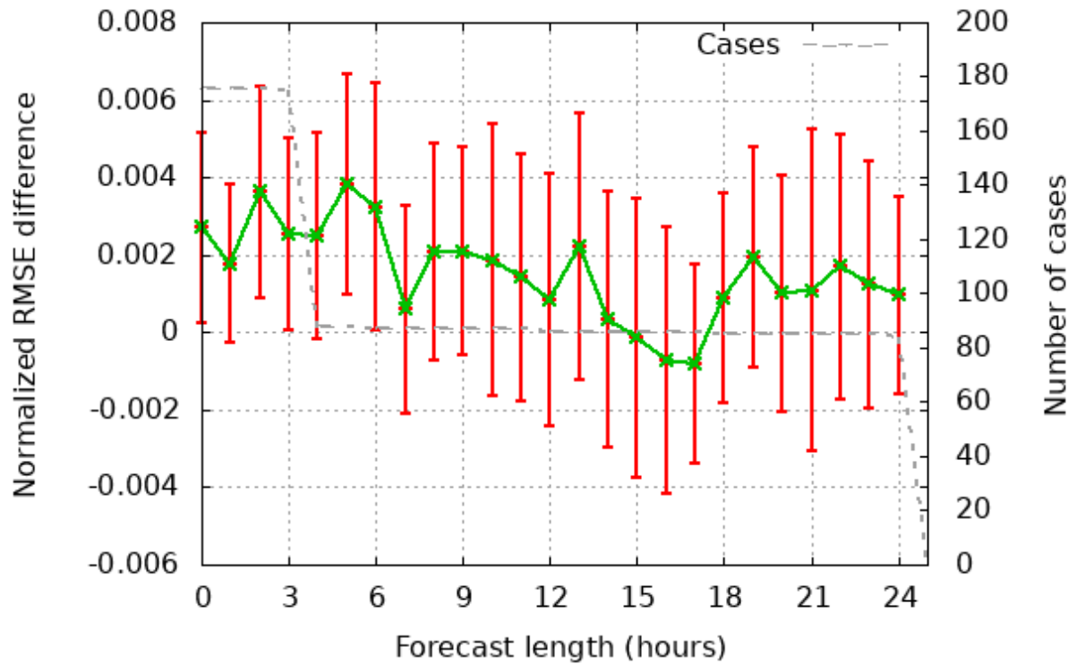
Figure 13. Significance test of normalized RMSE for relative humidity at 2 meters for Exp3 compared to Exp1. Positive values means smaller RMSE for Exp3 and thus a positive impact on the forecasts. The number of cases refers to the number of verification times.
