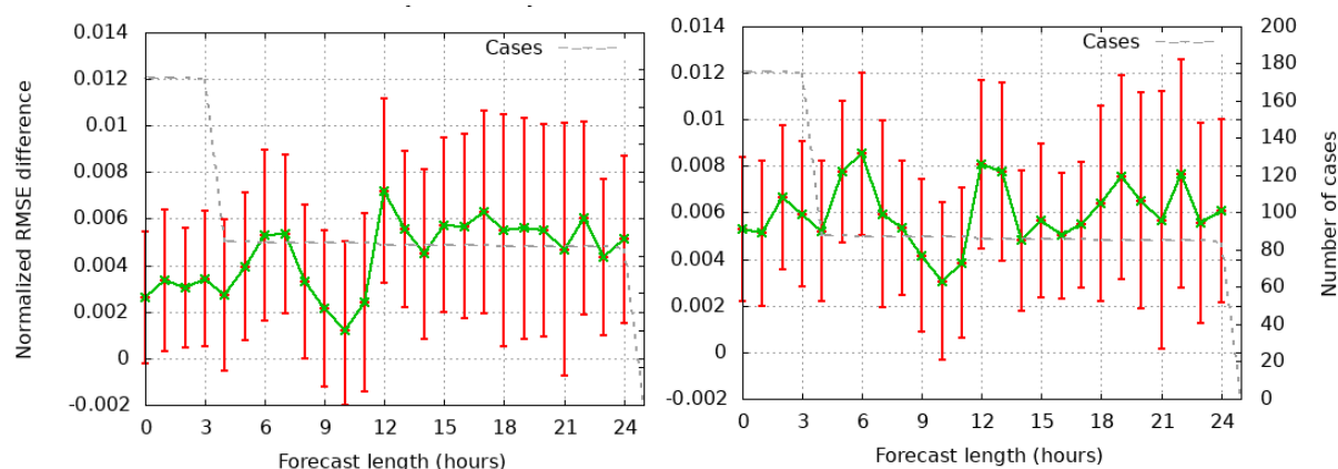
Figure 12. Significance test of normalized RMSE for relative humidity at 2 meters for Exp1 compared to the reference experiment (left) and for Exp3 compared to the reference experiment (right). Positive values means smaller RMSE for the radial velocity experiments and thus a positive impact on the forecasts. The number of cases refers to the number of verification times.
