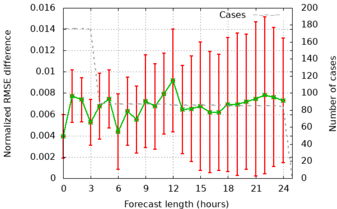
Figure 9. Significance test of normalized RMSE for mean sea level pressure for Exp3 compared to Exp1. Positive values means smaller RMSE for Exp3 and thus a positive impact on the forecasts. The number of cases refers to the number of verification times.
