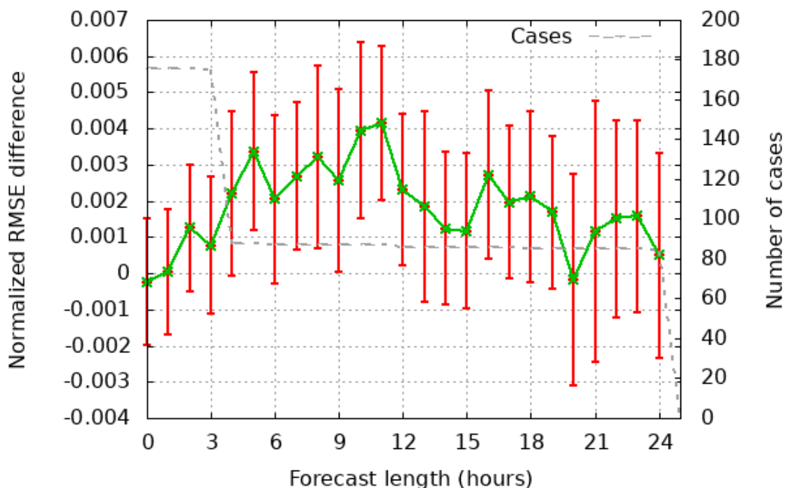
Figure 11. Significance test of normalized RMSE for temperature at 2 meters for Exp3 compared to Exp1. Positive values means smaller RMSE for Exp3 and thus a positive impact on the forecasts. The number of cases refers to the number of verification times.
