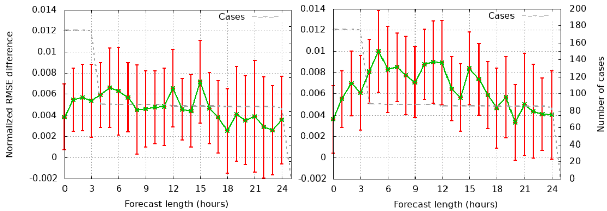
Figure 10. Significance test of normalized RMSE for temperature at 2 meters for Exp1 compared to the reference experiment (left) and for Exp3 compared to the reference experiment (right). Positive values means smaller RMSE for the radial velocity experiments and thus a positive impact on the forecasts. The number of cases refers to the number of verification times.
