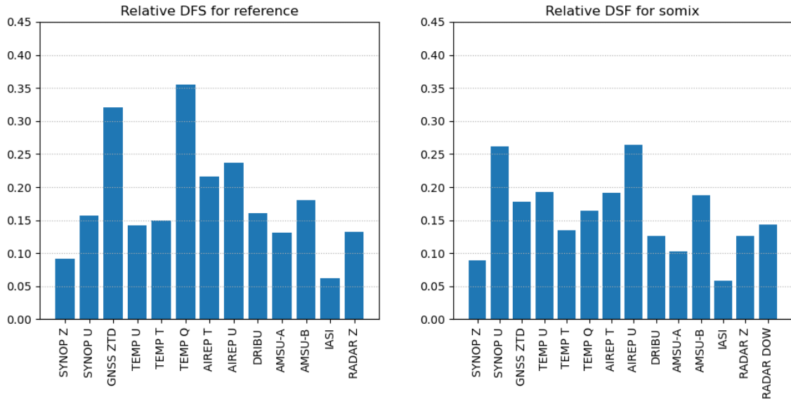
Figure 16. Relative DFS for the reference experiment (left) and the Exp3 (right) during a convective situation, 20210814 at 18.00 UTC.
