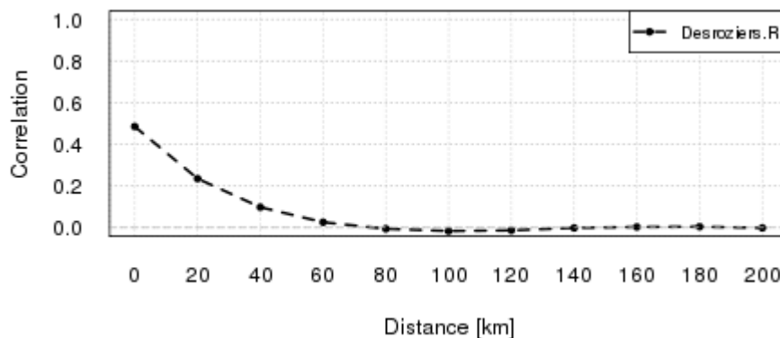
Figure 5. Spatial error correlation according to the distance between two radial velocity super observations derived using the Desroziers method.
