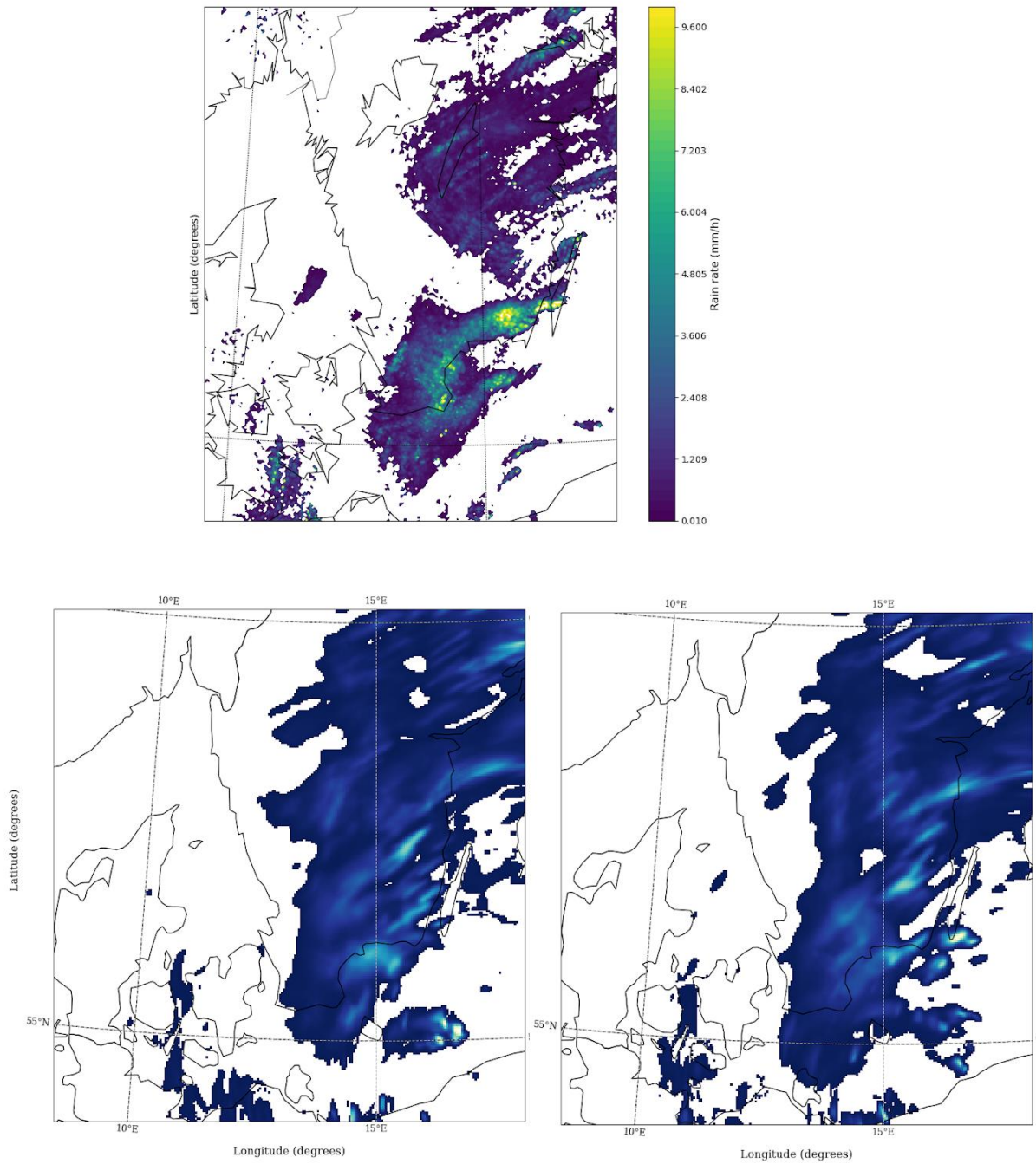
Figure 18. Upper panel: One hour accumulated precipitation radar image. Lower panels: One hour accumulated model precipitation from the reference run (left) and Exp3 (right). All are valid 20210826 at 18.00 UTC and the model accumulations are between forecast lengths 5 and 6 hours. The color scale is the same in all panels.
