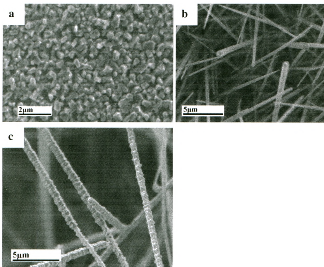
Figure 3. SEM images showing the effects of synthesis temperature on the nanostructures. a) Particles deposited on the substrate in temperatures at 900°C. b) Nanowires synthesized in 930°C. c) Nano & micro-wires synthesized in temperatures 960°C.
