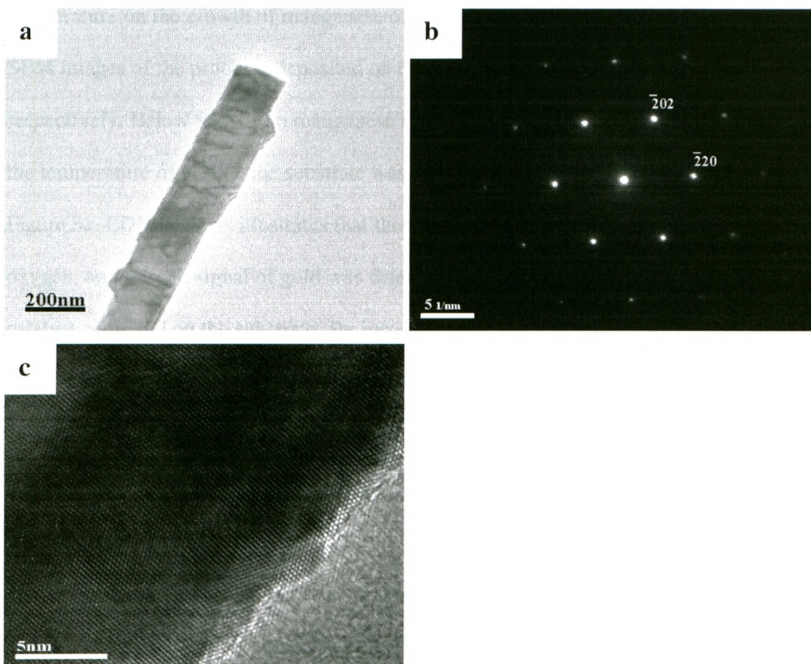
Figure 2. a) TEM image of a MnO nanowire with a diameter of about 150 nm. b) SAED pattern of the nanowires which corresponds to fcc-MnO phase. c) HRTEM image of manganese oxide nanowires.
