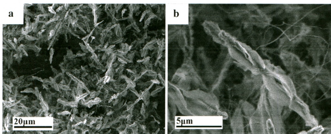
Figure 5. SEM images of structures synthesized by increasing the heating rate of the experiment to 50^{\circ}\text{C}/\text{min} while keeping other parameters at unchanged. a) low magnification SEM image shows that the composite structures cover the silicon substrate relatively uniformly. b) Higher magnification SEM images show that these structures are comprised of micro-wires in their core with sheet-like structures covering these wires. Initial characterizations via EDX show that the core wire is mainly composed of manganese and oxygen and the sheet covering the wire are mostly silicon oxide as seen in the EDX taken from these structures.
