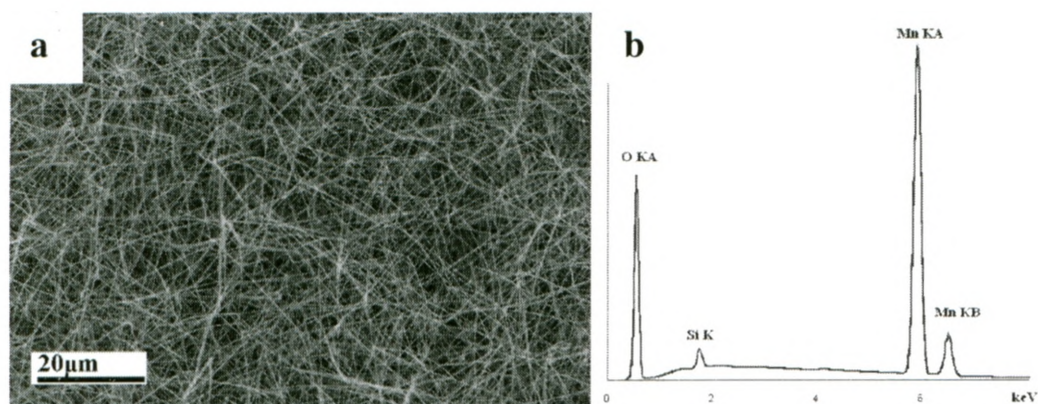
Figure 1. a) SEM images of manganese oxide nanowires synthesized on silicon substrate with 3-4nm, showing uniform coverage of silicon substrate. b) EDX spectrum of manganese oxide nanowires on silicon substrate with 3-4 nm gold.
