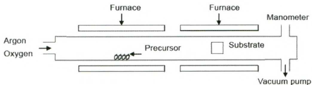
Figure 5. Schematic diagram of nanowires synthesized using a chemical vapor deposition method.
