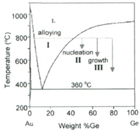
Figure2. Ge-Au Binary phase diagram [64].
