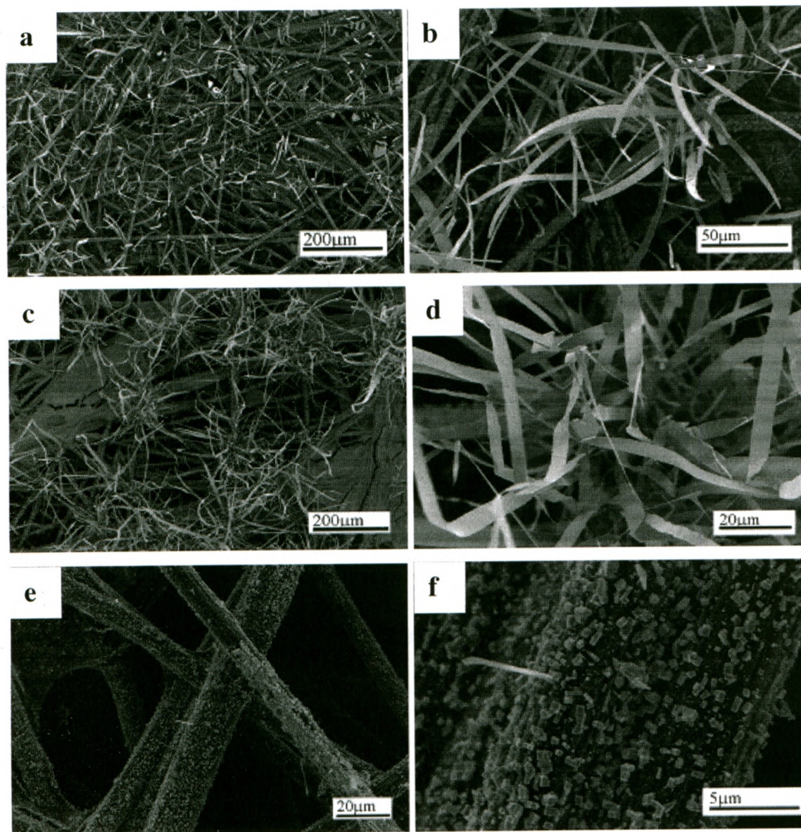
Figure 3. SEM images of MnO nanostructures synthesized on a,b) carbon paper, c,d) tungsten sputtered carbon paper, and e,f) titanium sputtered carbon paper in a catalyst free condition, revealing the dependence of the morphology of manganese oxide nanostructures on structure and composition of the substrate.
