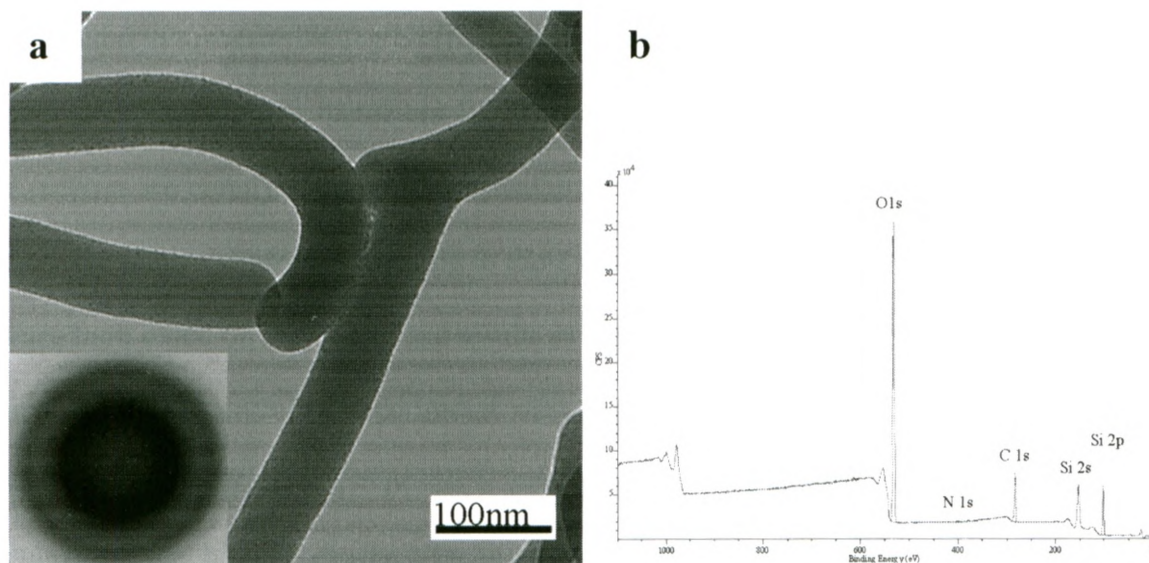
Figure 2. a) TEM image of silicon oxide nanowires showing smooth morphology and a diameter of 50-70 nm. The SAED pattern shown in the inset reveals a characteristic diffuse ring pattern indicating that silicon oxide nanowires are completely amorphous. b) XPS spectrum of silicon oxide nanowires with silicon to oxygen peak ratio of approximately 0.5, there were no peaks for \text{VO}_2 , suggesting that the nanowires are pure silicon oxide nanowires.
