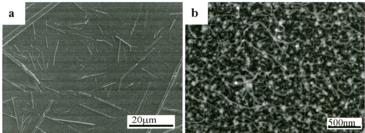
Figure3. SEM images showing the effect of hydrogen in the synthesis of silicon oxide nanowires. a) SEM image of vanadium oxide structures synthesized on silicon substrate by thermal annealing of silicon substrates in vicinity of VO_2 powder without the presence of H_2 in atmosphere. b) SEM image of low density of silicon oxide nanowires synthesized on silicon substrate coated with gold without the use of H_2 gas.
