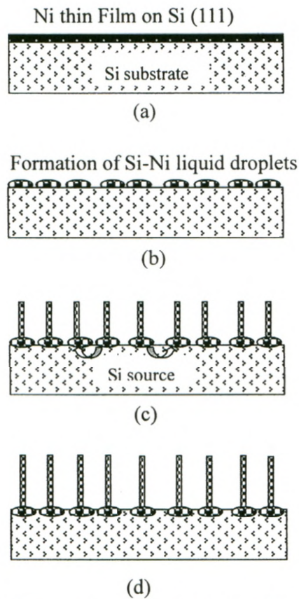
Figure4. Schematic diagram of Si nanowire synthesized using Ni catalyst via SLS growth mechanism [46].
