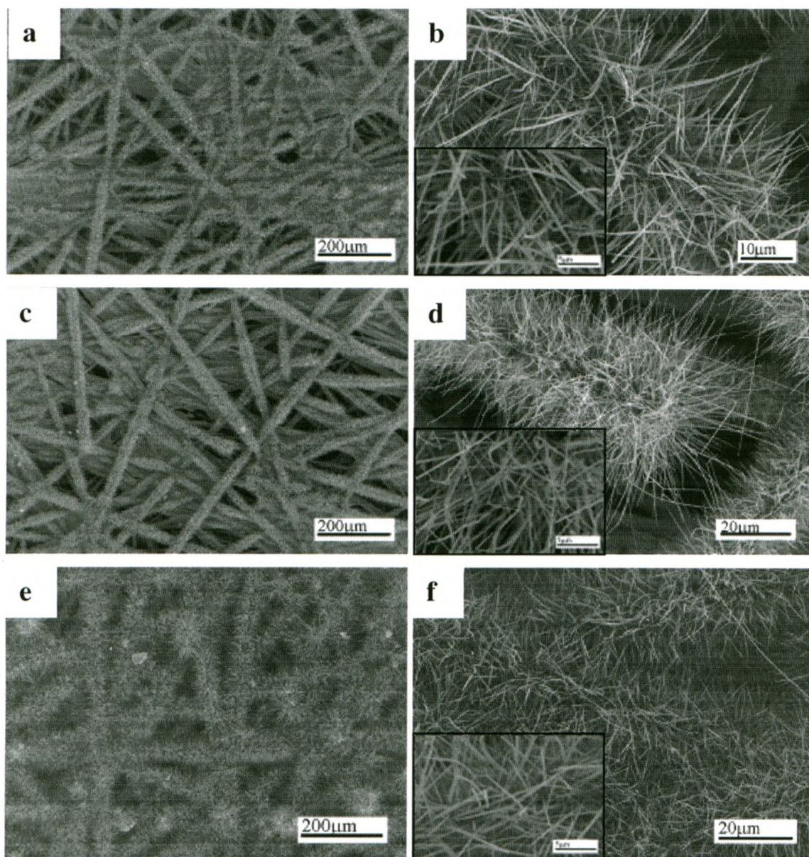
Figure 2. SEM images of MnO nanowires synthesized on carbon paper with a thin gold layer of a,b) 5nm, c, d) 10nm and e,f) 15nm showing the change in the morphology of nanowires deposited with the thickness of the catalyst layer.
