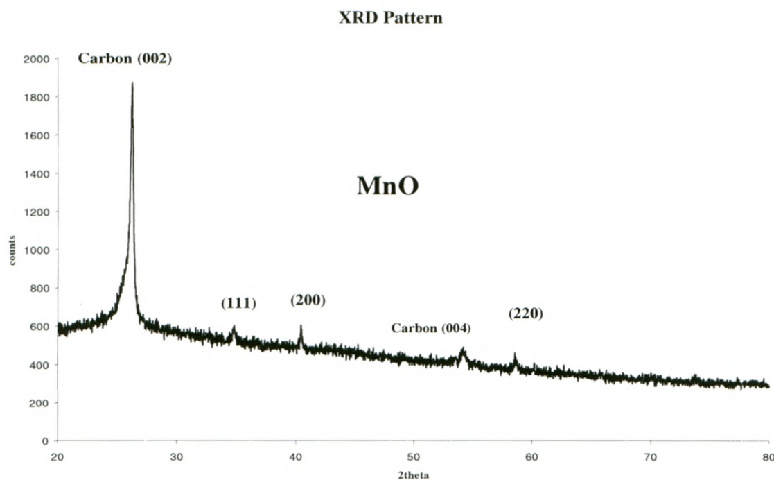
Figure1. XRD pattern from MnO nanowires synthesized on carbon paper with a 15nm thick gold layer.
