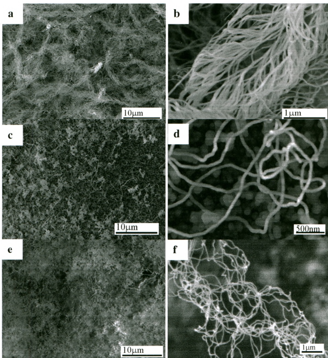
Figure 1. Typical SEM images of silicon oxide nanostructures synthesized using various catalysts by simple thermal annealing of silicon substrate. a) Low magnification of silicon oxide nanowires synthesized using the co-catalyst of \text{VO}_2 and Au. b) Increased magnification of silicon oxide network of nanowires synthesized using the co-catalysts. c) Low magnification of silicon oxide nanowires synthesized using gold catalyst. d) Increased magnification image of gold assisted grown silicon oxide nanowires with uniform diameter of these nanowires along their length with a with bundles of nanowires on the background. e) Low magnification image of silicon oxide nanowires synthesized using \text{VO}_2 as a catalyst. f) Increased magnification image of these silicon oxide network of nanowires.
