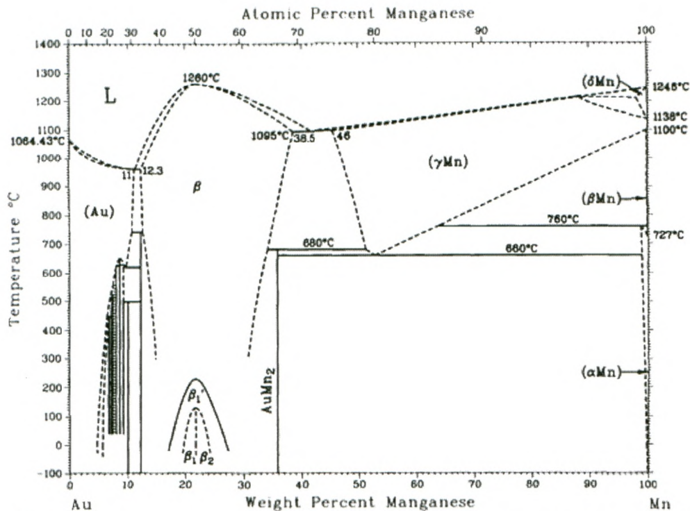
Figure3. Simplified binary phase diagram of Au-Mn, showing eutectic point around 960°C.
