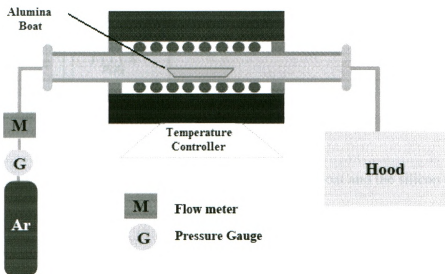
Figure2. Schematic diagram of CVD method used for the synthesis of manganese oxide nanostructures using manganese powder.
