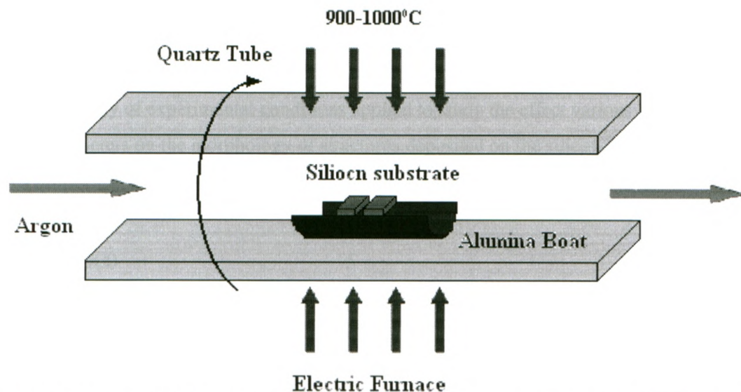
Figure4. Schematic diagram showing substrate-source setup in the quartz tube of CVD process for the synthesis of manganese oxide nanostructures on silicon substrate.
