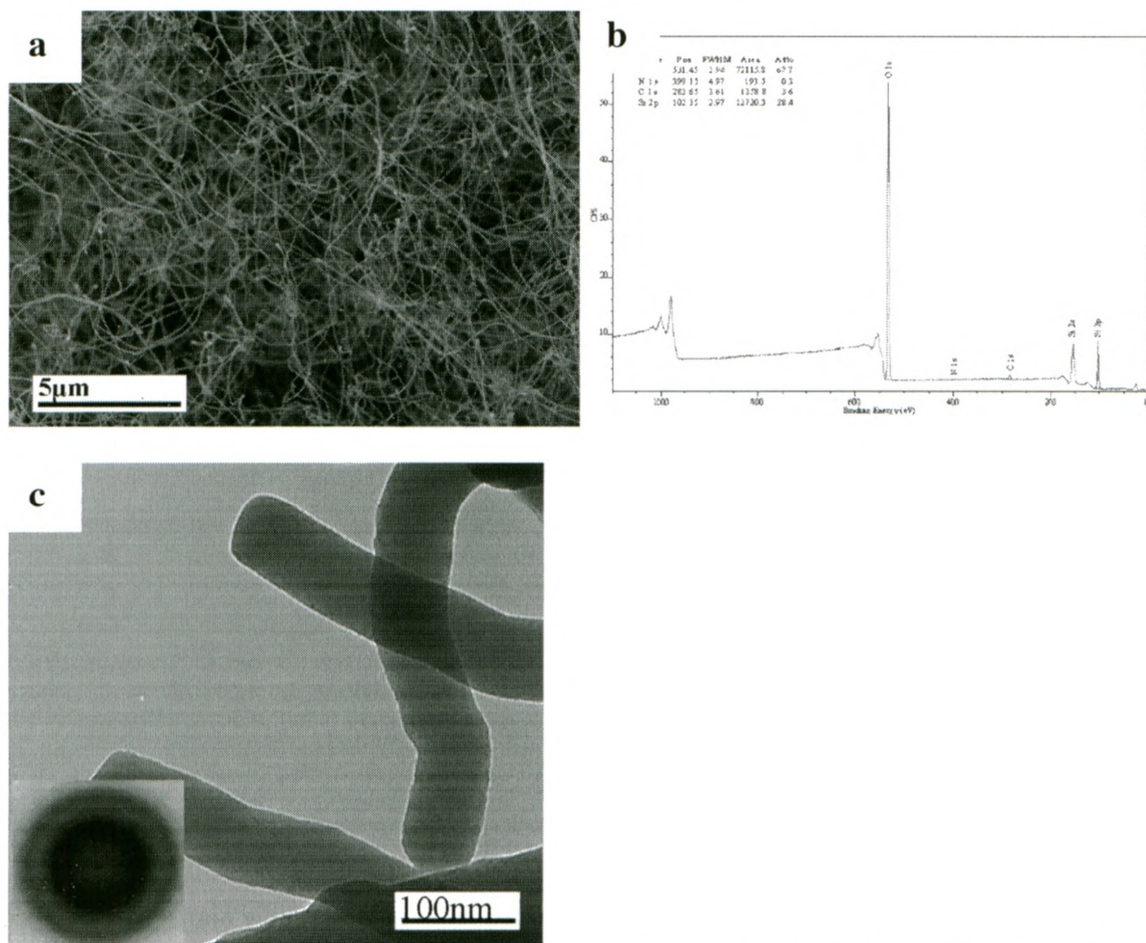
Figure 4. SEM images of silicon oxide nanowires synthesized by increasing the distance between manganese powder and silicon substrate to more than 5mm. a) SEM image of silicon oxide nanowires shows that these nanowires have uniform diameters below 100 nm and cover the substrate uniformly. b) XPS results from these nanowires shows that the Si:O ratio is around 1:2 which indicates that these nanowires are mainly \text{SiO}_2 nanowires. c) TEM image of silicon oxide nanowires showing smooth surface with narrow diameter range of 70nm. The inset is the SAED pattern of these nanowires taken under TEM reveals that these nanowires have amorphous structure.
