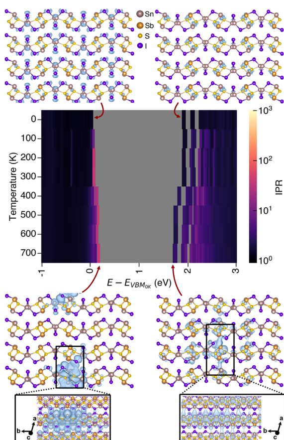
Figure 5. IPR of \text{Sn}_2\text{Sb}_2\text{I}_3 between 0 and 700 K, with the charge density isosurfaces (blue) of the VBM and CBM plotted for 0 and 700 K. Isovalue set to 5 \times 10^{-4} e/\text{\AA}^3 , and the atom colors are as follows: Sn = beige, Sb = orange, S = yellow, I = purple.
