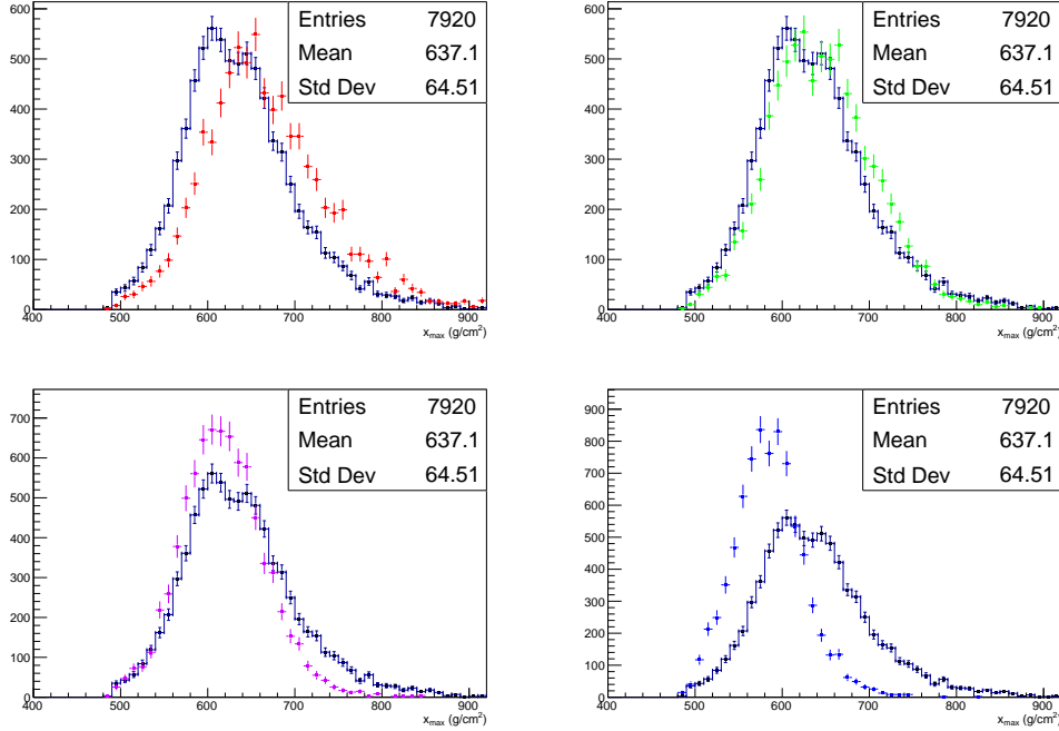
Figure 2: Shower X_{\max} ( \text{g}/\text{cm}^2 ) distributions for energy bin 16.7 < \log_{10}(E_{\text{cal}}/\text{eV}) < 16.8 . Each of four plots shows data histogram (black points / blue line), along with MC primary reconstructed X_{\max} : upper left plot H (red), upper right He (green), lower left CNO (violet), and lower right Fe (blue)
