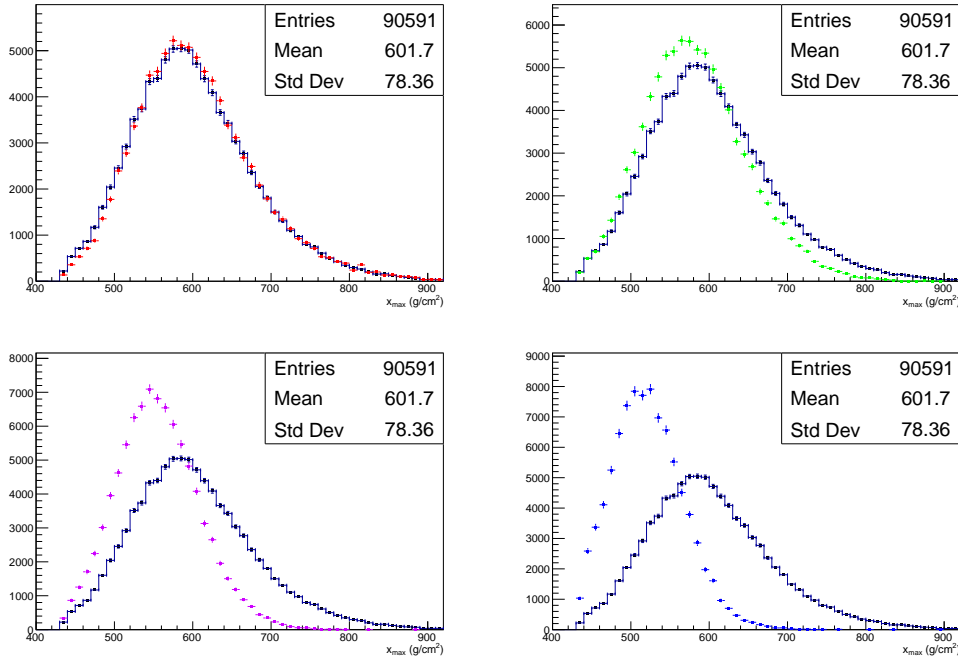
Figure 1: Shower X_{\max} ( \text{g/cm}^2 ) distributions for energy bin 15.7 < \log_{10}(E_{\text{cal}}/\text{eV}) < 15.8 . Each of four plots shows data histogram (black points / blue line), along with MC primary reconstructed X_{\max} : upper left plot H (red), upper right He (green), lower left CNO (violet), and lower right Fe (blue)
