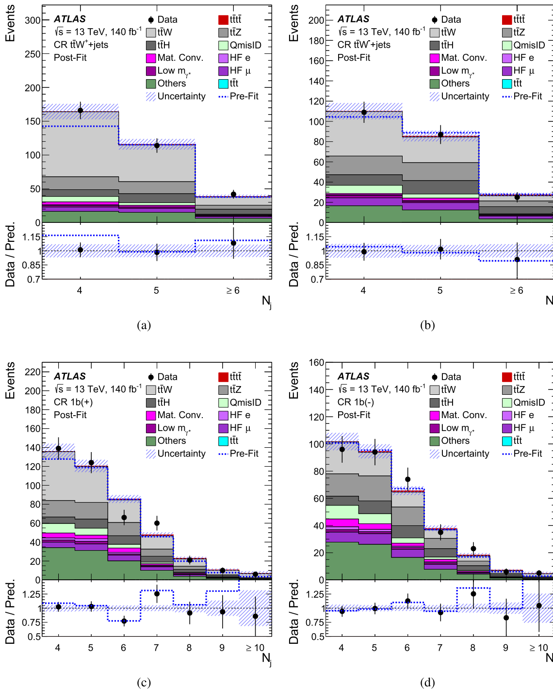
Fig. 2 Post-fit distributions for the number of jets ( N_j ) in each of the four t\bar{t}W CRs: a CR t\bar{t}W^+ + \text{jets} , b CR t\bar{t}W^- + \text{jets} , c CR 1b(+) and d CR 1b(-) . The ratio of the data to the total post-fit prediction is shown in the lower panel. The dashed blue lines show the pre-fit prediction in the
