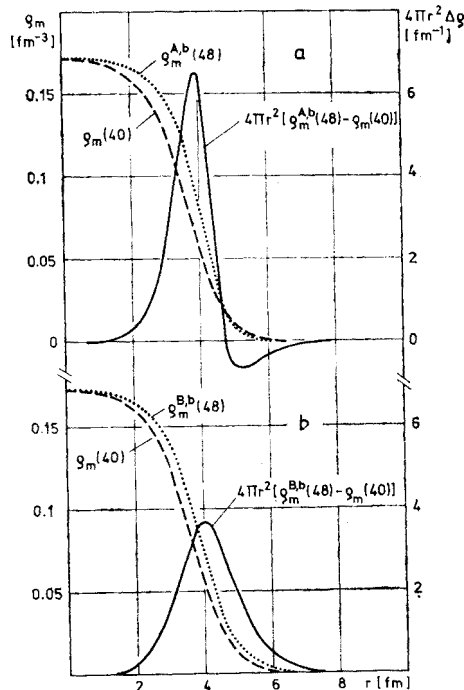
Fig. 1. Comparison of the matter density distribution \rho_m(40) of the ^{40}\text{Ca} nucleus (dashed line) with model matter density distributions \rho_m^{A,b}(48) and \rho_m^{B,b}(48) of the ^{48}\text{Ca} nucleus (dotted line) — see text. Radially weighted density difference is represented by solid line
