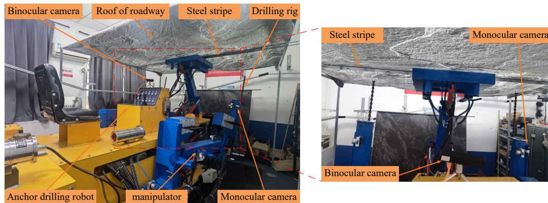
Figure 1. Anchor drilling robot.
