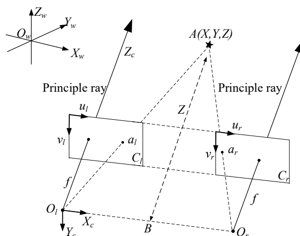
Figure 7. Model of binocular camera.
