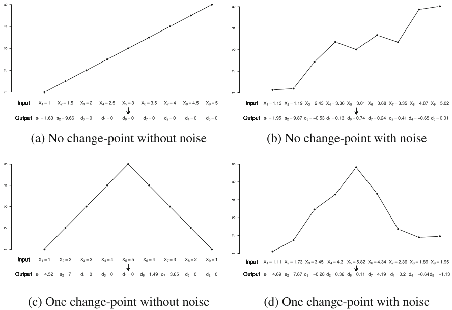
Fig. 1 Multiscale decomposition of the data through the TGUW transform when the data has no change-points (a, b) or one change-point (c, d). s_1 and s_2 are the smooth coefficients obtained through the TGUW transform and d_k is the detail coefficient obtained in the k^{\text{th}} merge. When the data has no noise (a, c), d_k = 0 for all k in a while two non-zero coefficients d_6 and d_7 encode the single change in c
