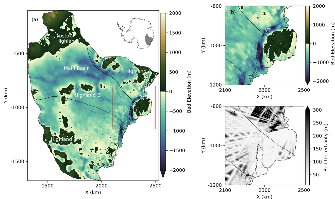
Figure 1. Aurora Subglacial Basin bed elevation and uncertainty derived from the BedMachine Antarctica v3 dataset (Morlighem et al., 2020). (a) Bed topography (m), with red zoom inset shown in panel (b), and (c) uncertainty (m). The ASB catchment outline is from Zwally et al. (2012) and the coastline and grounding line (black) are from MEaSUREs2. All data are referenced to the WGS84 ellipsoid and displayed in eastings (x-axis) and northings (y-axis) using polar stereographic coordinates (km). Locations of regions in panel (a) are: Vostok Highland; ASB main basin; Highland A; Highland B; Highland C; Sabrina Subglacial Basin (SSB); Totten Glacier (TG); Vanderford Glacier (VG); Sabrina Coast (SC); Knox Coast (KC); and the Elcheikh saddle point (black X). The Vanderford Trench (VT) is highlighted in panel (b).
