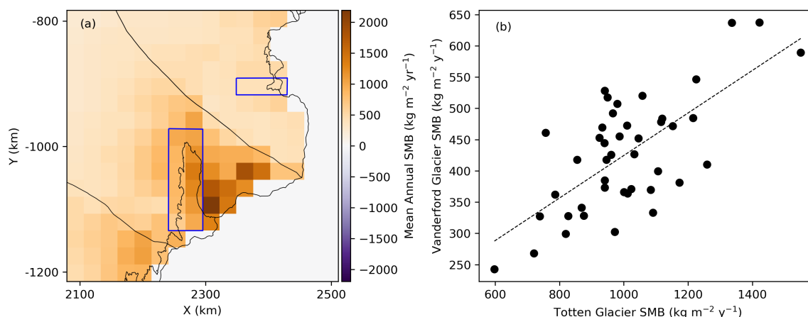
Figure 6. Surface mass balance over Law Dome and surrounding area. a) RACMO2.3p2 reanalysis (van Wessem et al., 2018) averaged over the period 1979 to 2021, showing a strong east-west snow accumulation gradient over Law Dome. Totten (larger) and Vanderford (smaller) bounding boxes for the SMB analysis in panel b are shown (blue). b) Vanderford annual snow accumulation as a function of Totten annual snowfall. Least-squares linear regression line shows slopes less than unity, indicating that for increasing local snow accumulation the mismatch between the Totten and Vanderford SMB is expected to increase.
