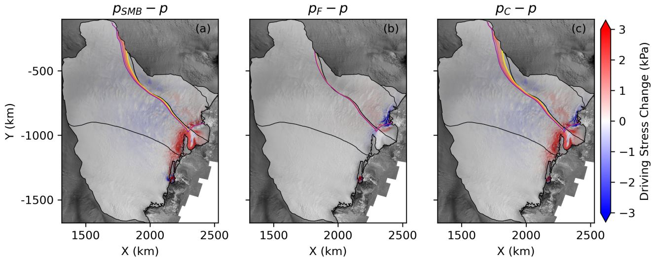
Figure 8. Driving stress changes (kPa) in the perturbation experiments for a 1°C increase compared with the control (m). (a) dS_{SMB} (expSMB 1 ), (b) dS_F (expFriction 1 ), and (c) dS_C (expCombined 1 ). The contours are the changes in the catchment divides for each of the perturbation experiments for 1 to 7°C, coloured brightest to dullest (yellow to purple), respectively.
