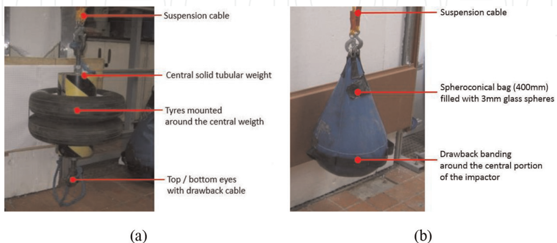
Figure 8. Conventional impactors for glass CWs: (a) twin-Tire and (b) Spheroconical bag (SB, with dimensions in mm) [61].
