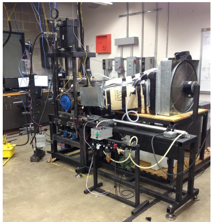
Figure 3. Single bearing tester (SBT) at UTRGV's UTCRS
