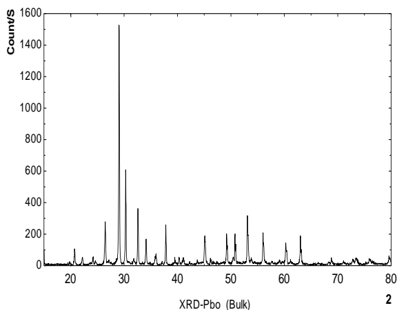
Fig .2. XRD Spectrum for Bulk sample of PbO
