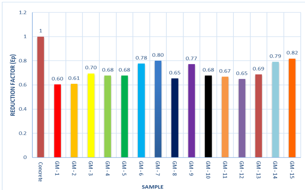
Figure 17. Reduction factor of peak interface friction angles (EP).
