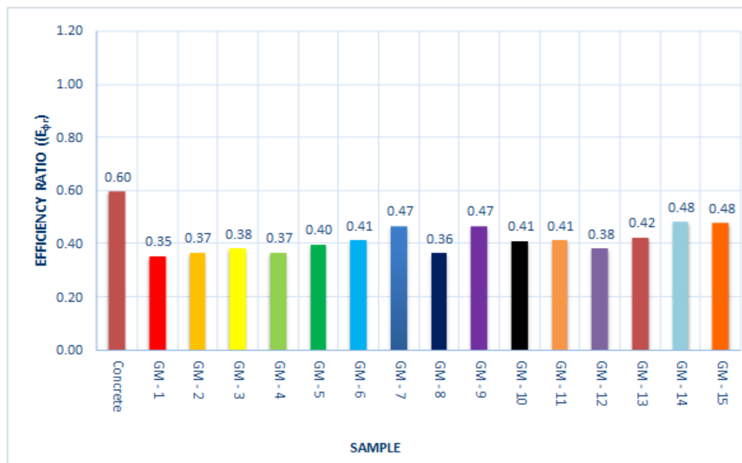
Figure 16. Efficiency ratio of peak residual friction angle (E \phi_r ).
