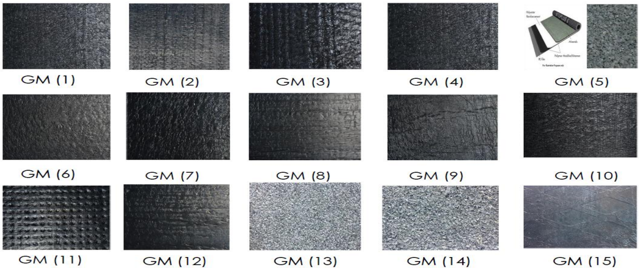
Figure 8. Geomembranes Samples.
