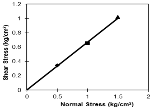
Figure 7. Direct shear test results of the sand soil.
