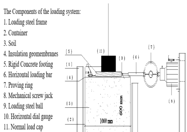
Figure 1. Schematic diagram for the model of modified direct shear test apparatus.
