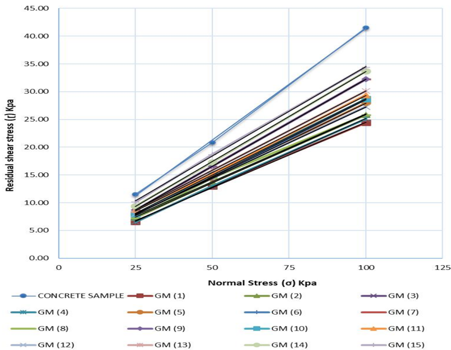
Figure 14. Normal stress and residual interface shear stress envelopes for both concrete and various geomembranes interfaces contacting with the sand.
