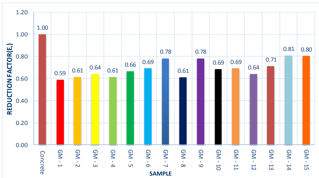
Figure 18. Reduction factor of peak interface friction angles (Er).
