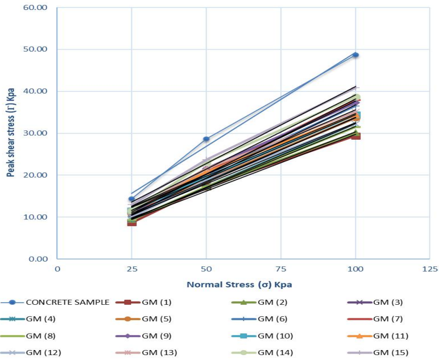
Figure 13. Normal stress and peak interface shear stress envelopes for both concrete and various geomembranes interfaces contacting with the sand.
