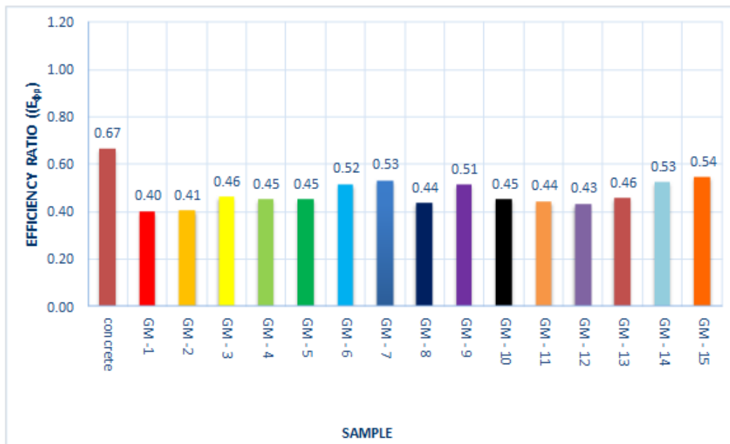
Figure 15. Efficiency ratio of peak friction angle (E \phi_p ).
