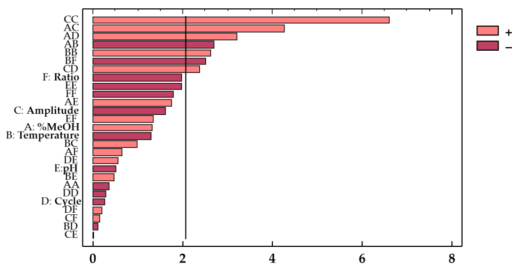
Figure 3. Standardized Pareto chart of the total phenolic compounds from red onion extracts.
