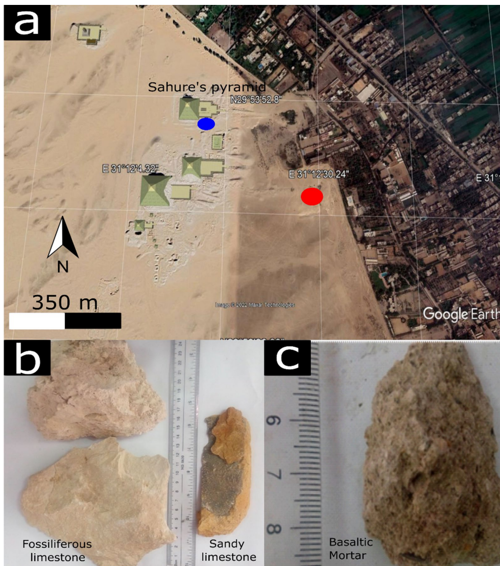
Fig. 6 a Image from Google Earth map showing the representative sampling areas for the construction material of the pyramid near Abusir village. The red circle refers to the local quarry from which the core blocks of the pyramid were extracted, and in the blue circle, the place where some fragments were collected from fallen and highly weathered fragments/samples. These fragments represent the fossiliferous limestone as casing stone and sandy limestone as core building material (b) and the mortar fragment (c)
