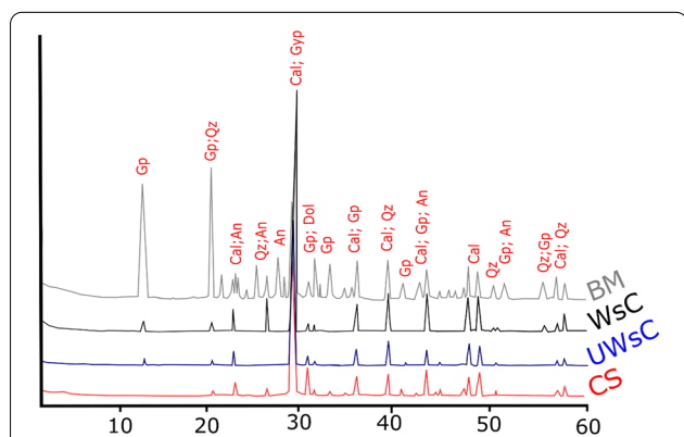
Fig. 10 X-ray diffraction patterns of the construction materials of Sahure’s pyramid. Legend: CS, core stone; UWsC, unweathered casing stone; WsC, weathered casing stone; BM, basaltic mortar; Gyp, gypsum; Qz, quartz; Cal, calcite; An, anorthite; Dol, dolomite (according to Ref. [70])
