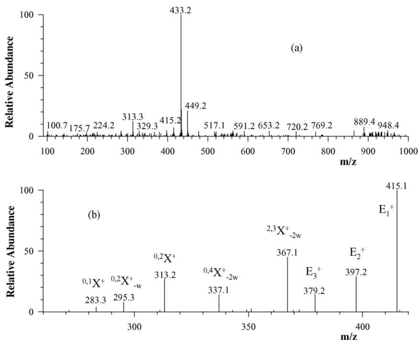
Fig. 5. (a) Mass spectrum at retention time 56 min in the LC-chromatogram of the extract (see Fig. 2). [M + H]^+ ion at m/z 433 corresponds to compound 1 . (b) MS/MS spectrum for the parent ion m/z 433.
