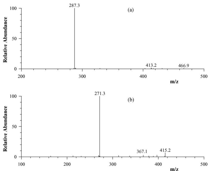
Fig. 4. MS/MS for the [M + H]^+ ions of (a) compound 2 and (b) compound 3 .
