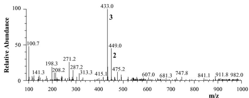
Fig. 3. Mass spectrum at retention time 62 min in the LC-chromatogram of the extract (see Fig. 2). [M + H]^+ ions at m/z 449 and 433 correspond to compounds 2 and 3 , respectively.
