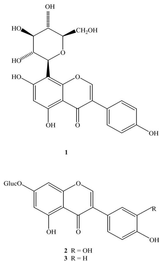
Fig. 1. Structure of the flavonoid glycosides 1–3.
