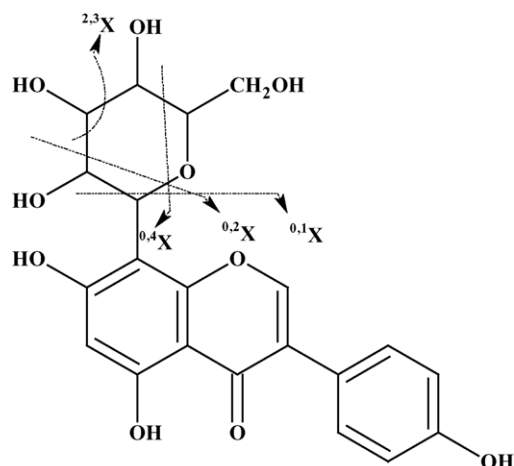
Fig. 6. Proposed structure for compound 1 indicating some fragmentations occurred by ESI–MS/MS.
