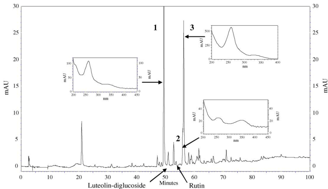
Fig. 2. Chromatogram of the extract detected at 280 nm and UV spectra of the compounds identified as genistein-8- C -glucoside (peak 1, RT = 49.5 min), luteolin-7- O -glucoside (peak 2, RT = 56 min) and genistein-7- O -glucoside (peak 3, RT = 56.4 min).
