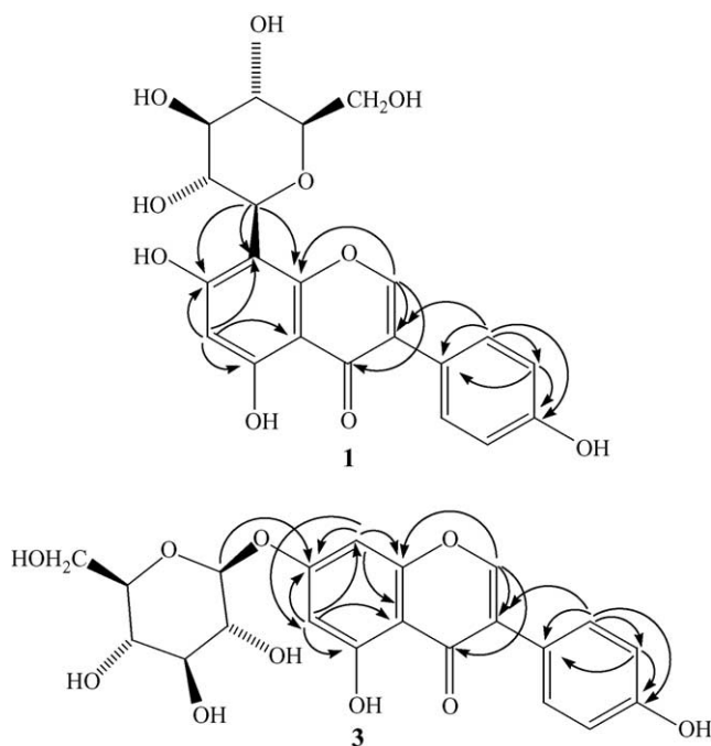
Fig. 7. Important HMBC correlations for the structure elucidation of compounds 1 and 3 .
