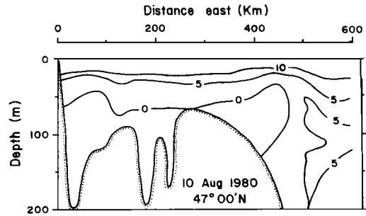
FIGURE 2. Thermal profile across the Avalon Channel and Grand Banks during the summer. Redrawn from Hollibaugh and Booth (1981).
