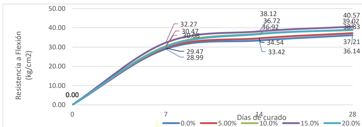
Fig. 23: Mortero, 0%, 5%, 10%, 15% y 20% Residuos de Ladrillo
