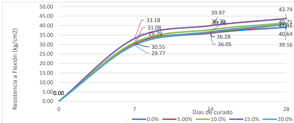
Fig. 22: Mortero, 0%, 5%, 10%, 15% y 20% Residuos de Ladrillo
