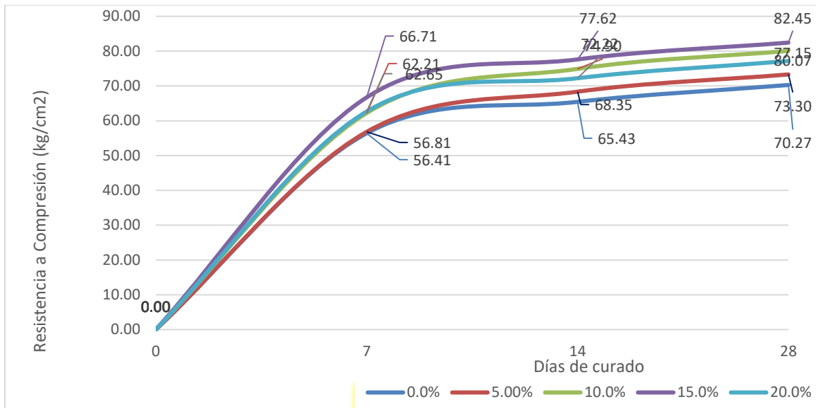
Fig. 18: Mortero, 0%, 5%, 10%, 15% y 20% Residuos de Ladrillo
