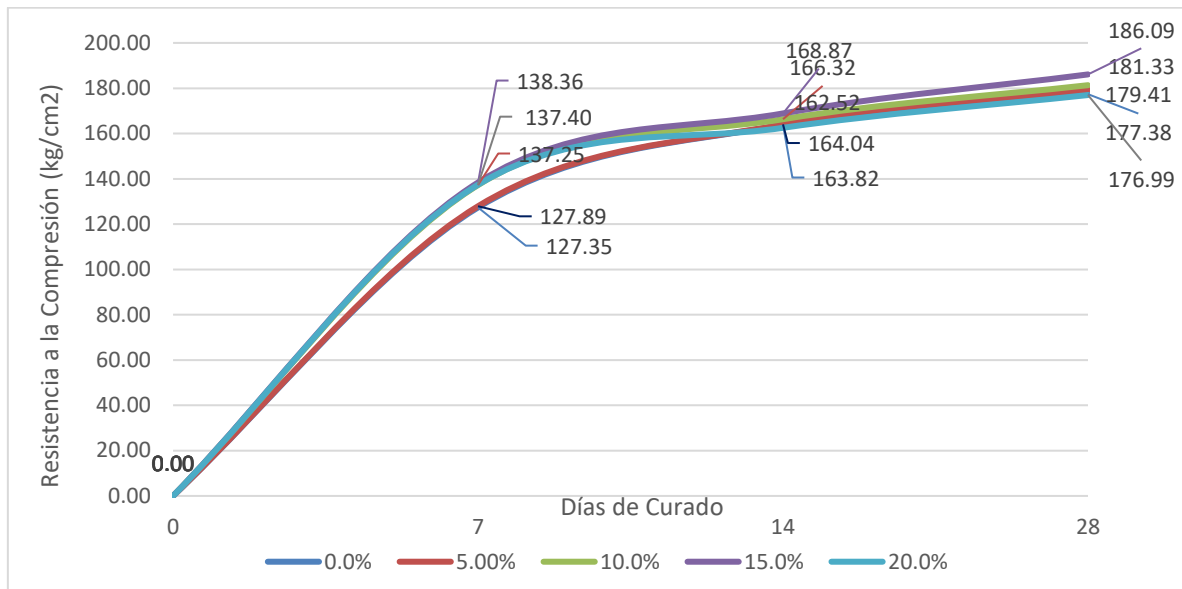
Fig. 16: Mortero, 0%, 5%, 10%, 15 y 20% Residuos de ladrillo
