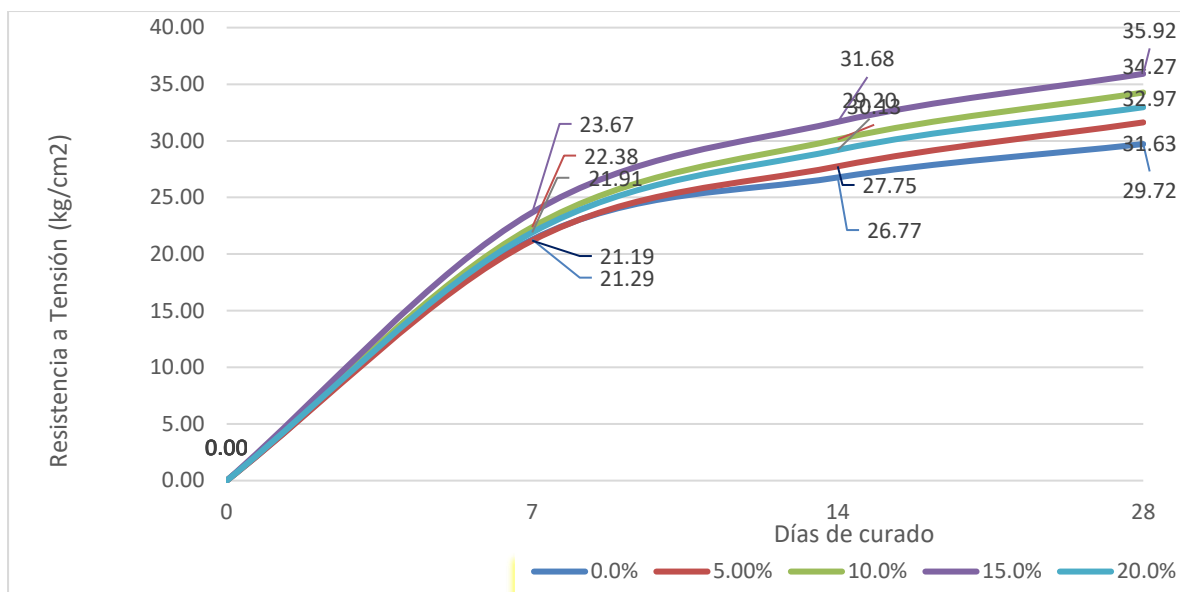
Fig. 19: Mortero, 0%, 5%, 10%, 15% y 20% Residuos de Ladrillo
