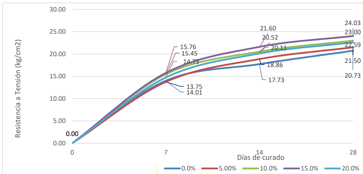
Fig. 21: Mortero, 0%, 5%, 10%, 15% y 20% Residuos de Ladrillo
