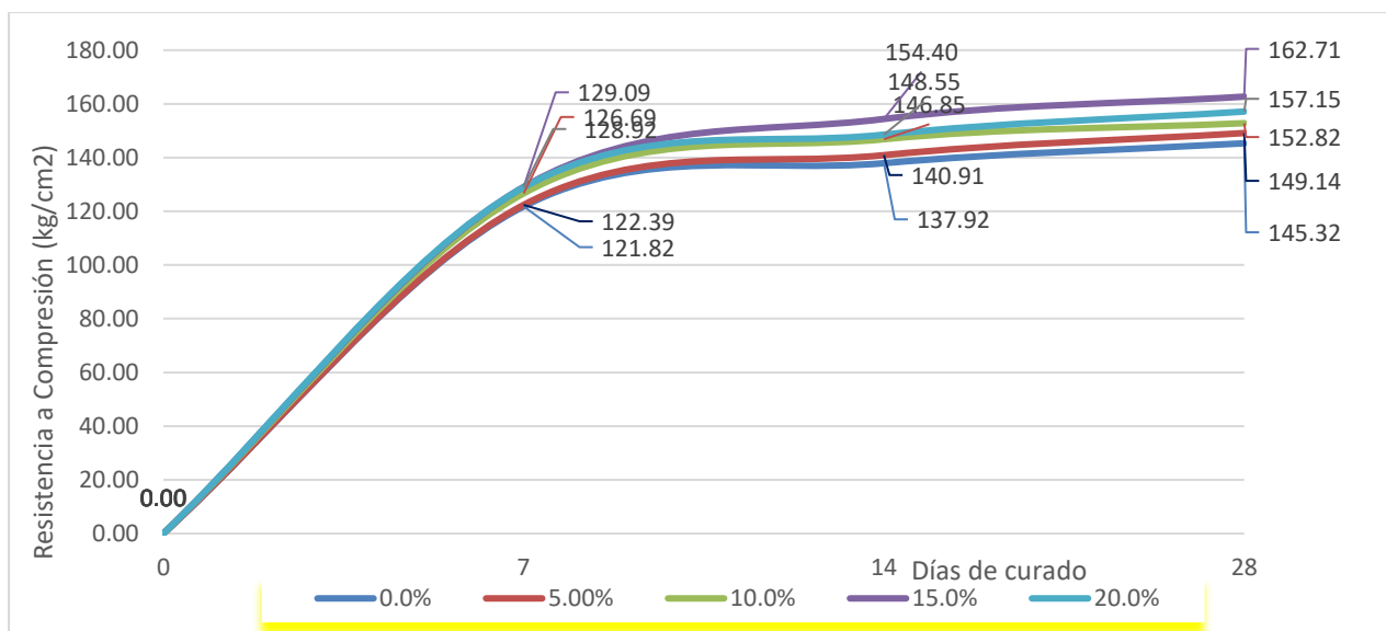
Fig. 17: Mortero, 0%, 5%, 10%, 15% y 20% Residuos de Ladrillo
