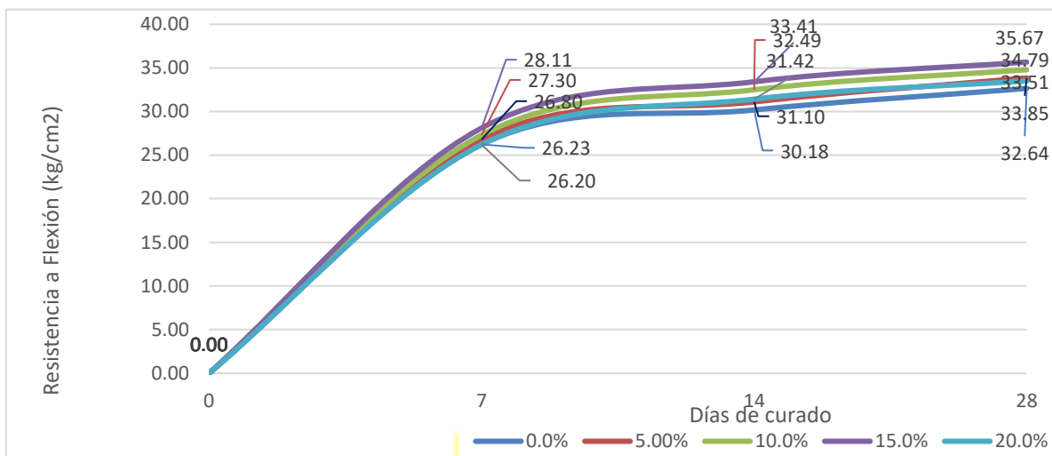
Fig. 24: Mortero 0%,5%, 10%, 15% y 20% Residuos de Ladrillo
