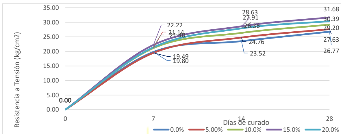
Fig. 20: Mortero, 0%, 5%, 10%, 15% y 20% Residuos de Ladrillo
