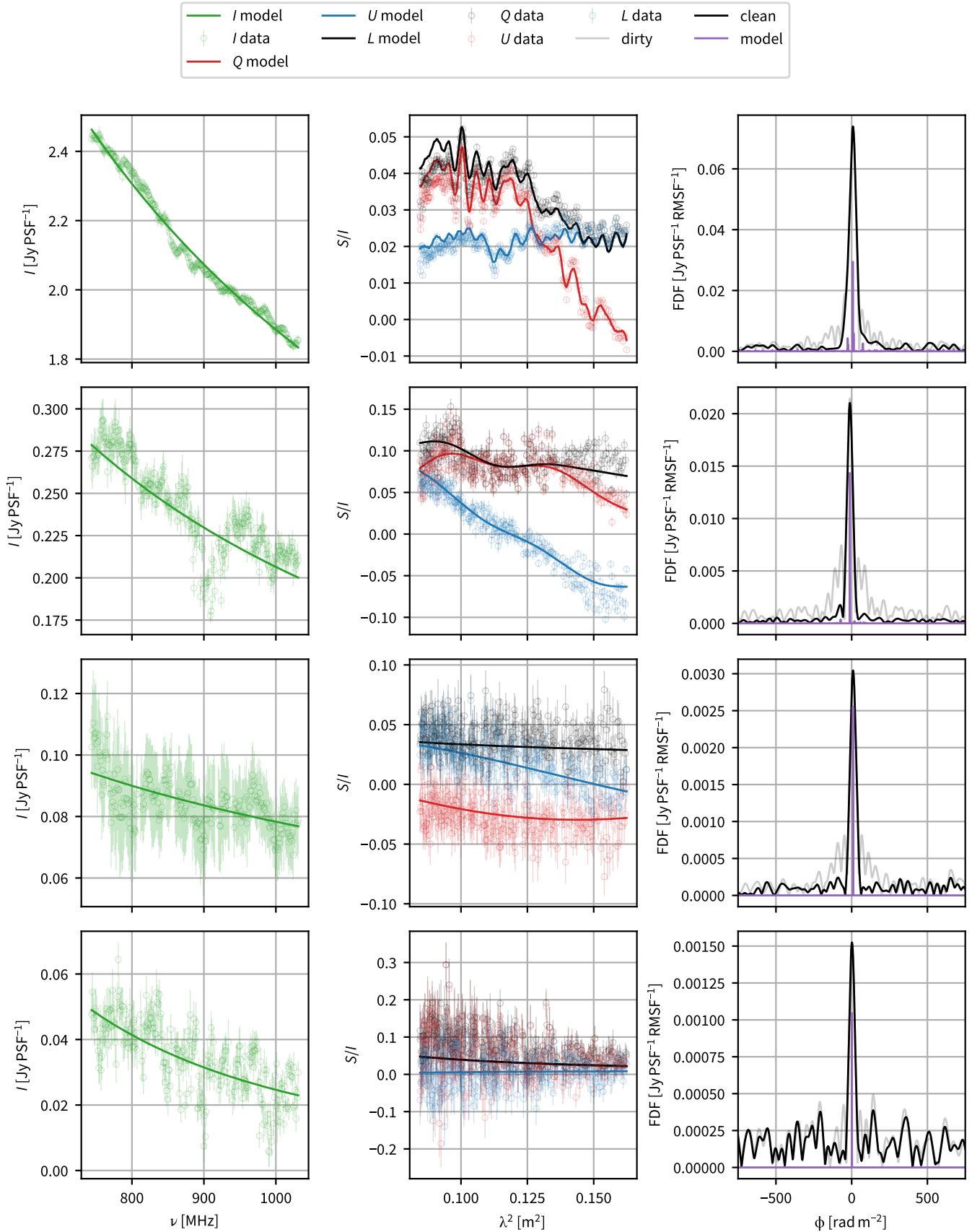
Figure 17. Example spectra of four sources from SPICE-RACS nearest to the 99.9 ^{\text{th}} , 97.7 ^{\text{th}} , 84 ^{\text{th}} , and 50 ^{\text{th}} percentile in polarised signal-to-noise from top to bottom. In the left column we show the Stokes I data and our fitted power-law model. In the middle column we show the fractional Stokes Q and U , and polarised intensity L . Here the scatter points are the observed data divided by the Stokes I model, and the solid lines is the RM-CLEAN model transformed to \lambda^2 space. In the right-hand column we show the dirty, clean, and model Faraday dispersion functions (FDFs) in polarised intensity.
