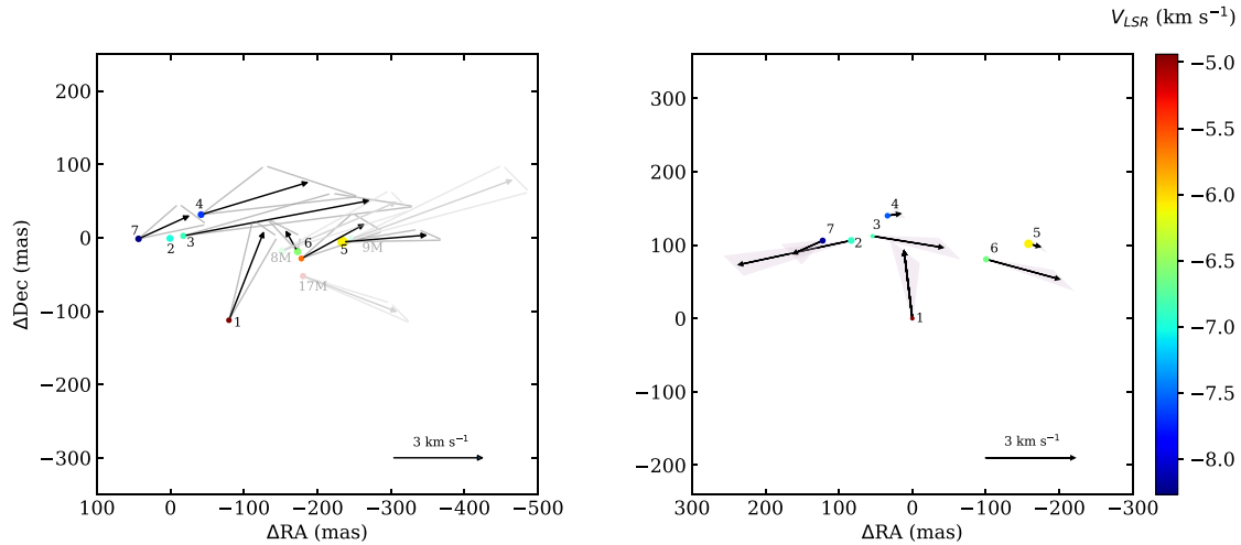
Figure 5. Relative proper motions of 6.7 GHz maser cloudlets in G78. Left: Results for the model of the disc-jet interface scenario by Moscadelli et al. (2011a), over a period of 2004–2019. The numbers correspond to the names of persistent cloudlets as given in Table B1. The light-coloured circles and light grey vectors correspond to features 8, 9, and 17 from Table 1 in Moscadelli et al. (2011a); they were not detected in 2011 and 2019. The grey triangles correspond to the uncertainties of proper motion vectors. Right: Relative proper motions derived from distance changes between cloudlet pairs as described in Section 5.2.
