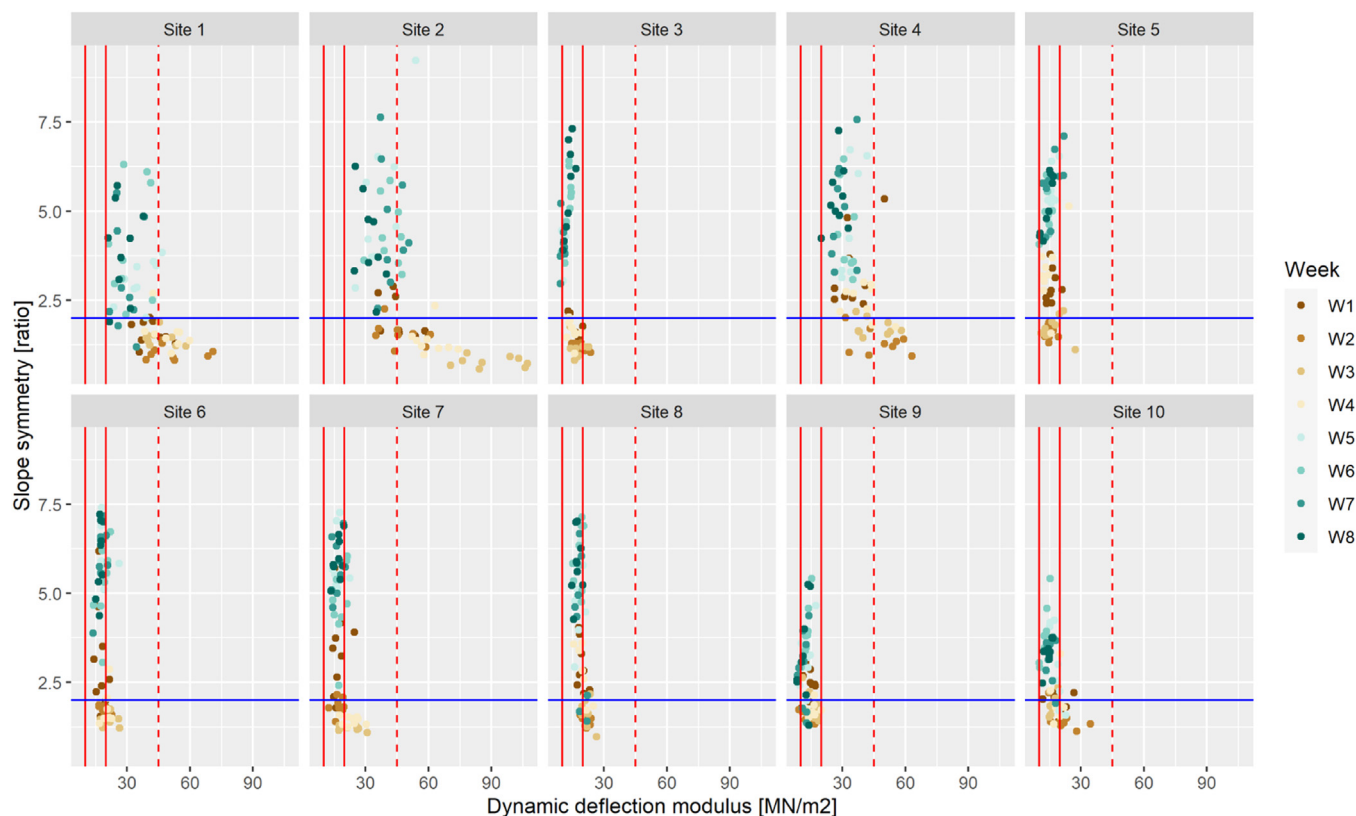
Fig. 8. Dynamic deflection modulus ( E_{vd} , \text{MN/m}^2 ) plotted against slope symmetry ratio colored by week of measurement (vertical solid red line: ideal E_{vd} 10–20 \text{MN/m}^2 , vertical dashed red line: E_{vd} = 40 \text{MN/m}^2 , horizontal solid blue line: slope symmetry ratio = 2). Hard surfaces rarely exhibit slope symmetry ratios larger than two while soft surfaces' symmetry ratios show a larger variation.
