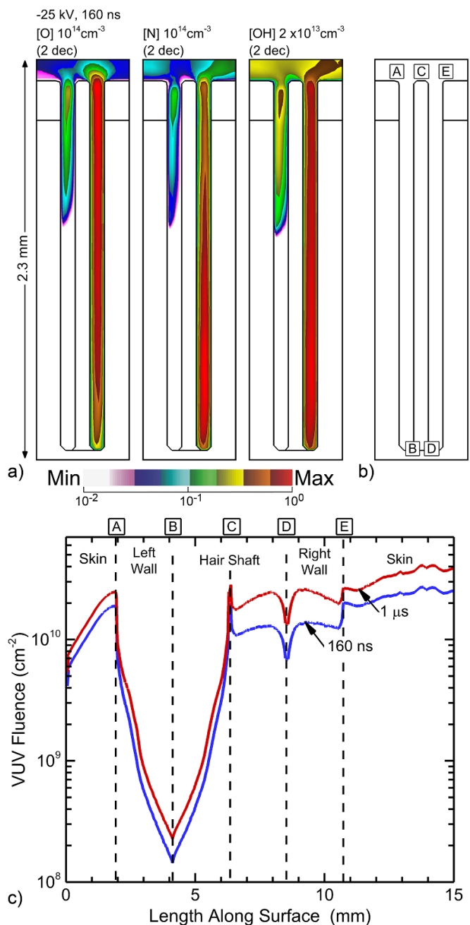
Figure 8. Radical and photon properties in the follicle. (a) Densities of O, N and OH at the end of the voltage pulse at 160 ns. Images are plotted on a 2 decade log-scale with the maximum value noted in each frame. (b) Reference locations for photon fluences. (c) VUV photon fluences to the inside surfaces of the follicle at 160 ns (end of voltage pulse) and 1 \mu\text{s} . The locations along the surface of the follicle are indicated by the boxed letters.
