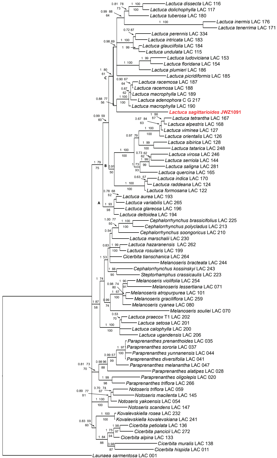
Figure 2. Majority consensus phylogram of the Lactucinae from Bayesian analysis (support values: first line Bayesian posterior probability / maximum likelihood bootstrap; second line maximum parsimony jackknife) based on the nrITS region.
