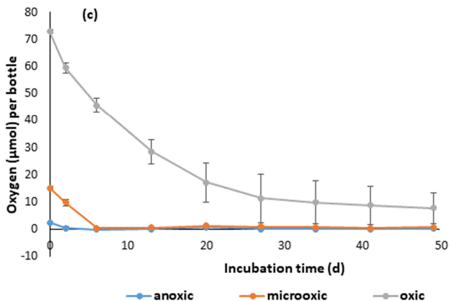
Figure 4. (a) Cumulative net N 2 O reduction; (b) cumulative net CO 2 production; and (c) O 2 depletion by strain IGB 4-14 T under anoxic, microoxic (4% O 2 ) and oxic (20% O 2 ) conditions. The plotted values are averages of six repetitions, corrected by the average of three controls. Error bars represent the standard deviations. Different letters indicate significant differences ( p < 0.05 ).
