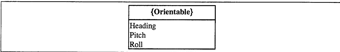
Figure 39. The ObjectSim 3.0 API Orientable Entity Class
