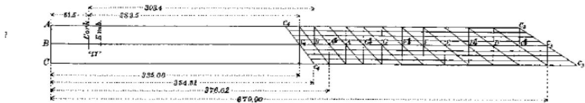
FIG. 12. Schema for determining the positions of the tone-holes of wind Instruments at various pitches.
