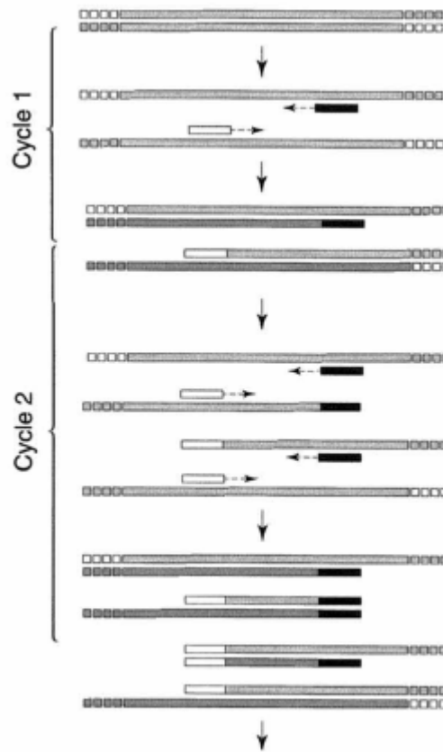
Figure 1. Exponential amplification of a single template molecule of DNA during PCR. Each cycle consists of a denaturation, annealing, and elongation stage (McPherson & Møller, 2000).
