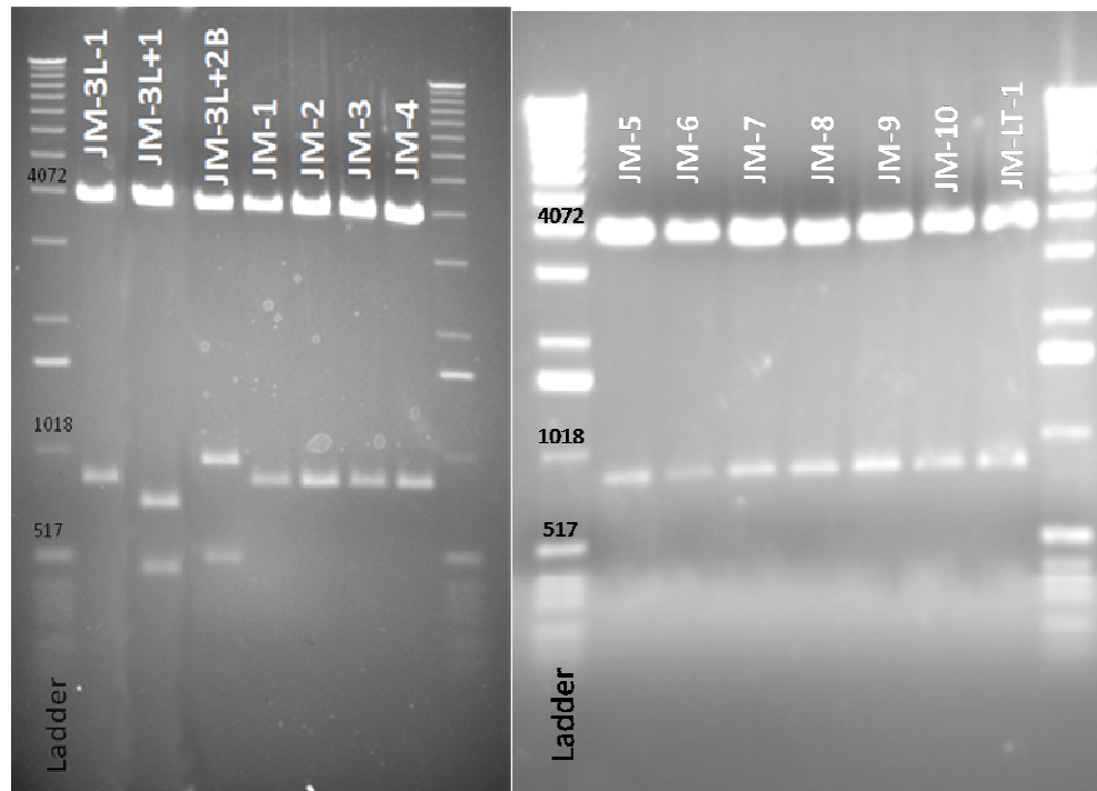
Figure 9. Restriction digest with EcoRI on a 1.0% agarose gel. (Mayhew, 2008)
