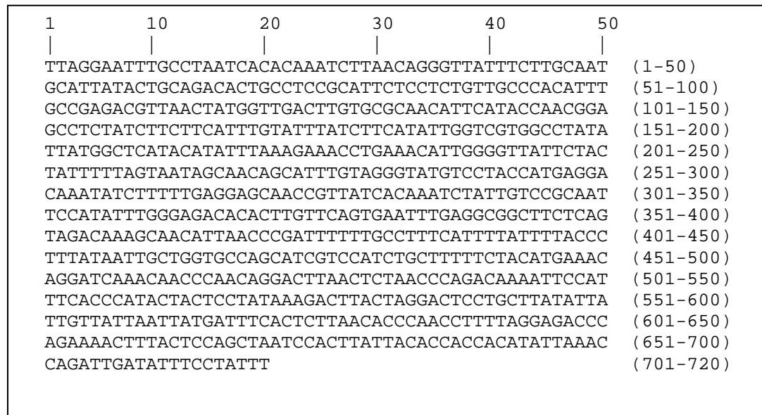
Figure 5. Consensus sequence of eleven salamander larvae exhibiting high levels of similarity (99.0%).
