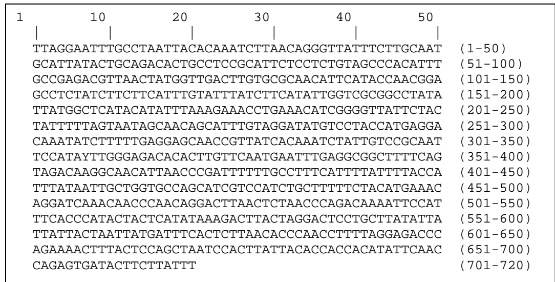
Figure 6. Consensus sequence of ten E. lucifuga from Franklin County, Tennessee. (Zigler & Harlan, 2006).
