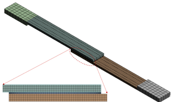
Fig. 3. The mesh of Al-CFRP single lap sample. Only half of the geometry was considered, resulting in approximately 50 k nodes.
