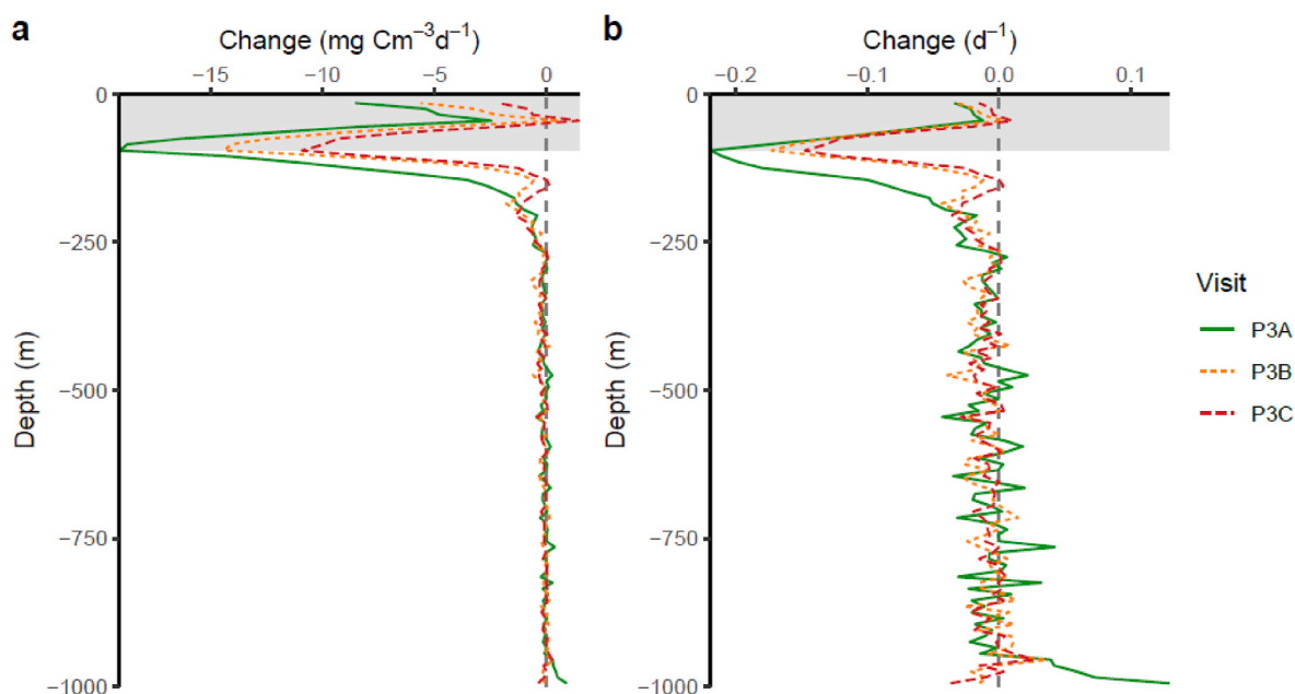
Fig. 8. Change in vertical POC flux with depth during each visit expressed as (a) absolute mass ( \text{mg C m}^{-3} \text{d}^{-1} ), and (b) fraction of POC concentration at that depth ( \text{d}^{-1} ). I.e. the value at 250 m refers to the change of POC flux from 249 m depth to the flux at 250 m depth. Visits P3A, P3B and P3C are shown in solid green, dotted orange and dashed red, respectively. The mixed layer is shaded in grey.
