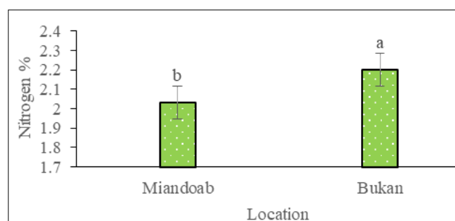
Fig. 1. Comparison of the two studied locations in terms of the root nitrogen content.
