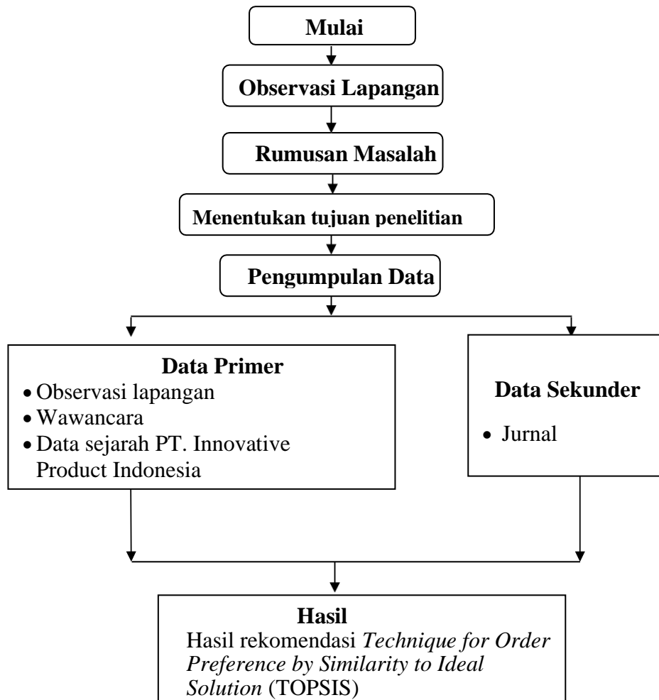
Gambar 1 Flowchart Penelitian
