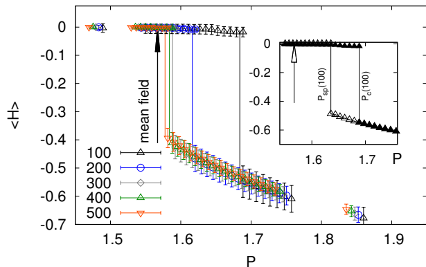
FIG. 1: (Color online) Energy vs. \mathcal{P} (in arbitrary units) in the Frequency Comb case with N_q \propto N^2 . The arrow marks the analytic critical point in the thermodynamic limit of the NBT. Inset: for N = N_f = 100 modes the spinodal line \mathcal{P}_{sp} is shown next to the threshold critical line.
