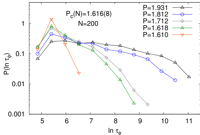
FIG. 5: (Color online) Distribution of the decay time of the equal time phase correlation function for a system of N = N_f = 200 modes across the threshold \mathcal{P}_c(N = 200) = 1.616(8) . Time \tau in is Monte Carlo steps.
