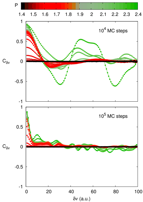
FIG. 6: (Color online) Phase-Phase correlation C_{\delta\nu}(\mathcal{T}) as function of frequency difference \delta\nu = \nu' - \nu and optical power \mathcal{P} for \mathcal{T} = 10^4 (top panel) and \mathcal{T} = 10^5 (bottom panel) in a FCT cavity with N = 100 and N_q = \mathcal{O}(N^2) . The threshold power is \mathcal{P}_c(100) = 1.62(2) and the range of power of the displayed correlations is reported on the top palette from black (black online) for low power to light grey (light green online) for high power.
