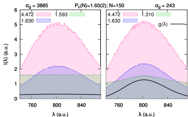
FIG. 3: (Color online) Intensity spectra for a FCT system of N_f = N = 150 . N_q = \mathcal{O}(N^2) for increasing \mathcal{P} from bottom to top. Left: gain g(\lambda) with larger variance, \sigma_\lambda = 3885 . At \mathcal{P} > \mathcal{P}_c the spectrum starts narrowing because of the nonlinear mode-coupling. Right: g(\lambda) with smaller variance, \sigma_\lambda = 243 . Spectra follow the peaked gain profile already in the CW regime. At \mathcal{P}_c mode-locking sets in, enhancing the sharpening.
