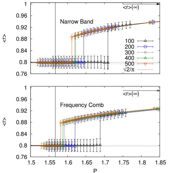
FIG. 2: (Color online) Average mode magnitude r = \langle |a| \rangle / \sqrt{\epsilon} vs. optical power \mathcal{P} (in a. u.) for different sizes in the NBT (top panel) and in the FCT (bottom panel).
