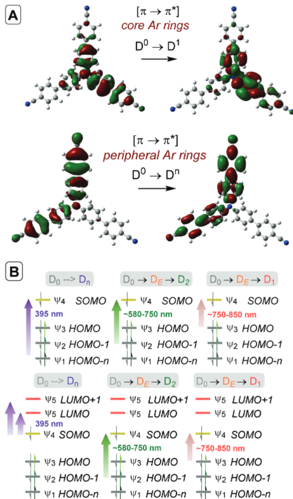
Fig. 15 (A) Natural Transition Orbitals (NTOs) depicting photoexcitation of \text{TCBPA}^+ to D_1 or D_n . (B) TD-DFT predicted orbital transitions of \text{TpBPBA}^+ (top) and \text{TCBPA}^+ (bottom). Wavelengths are derived from optical transitions.
