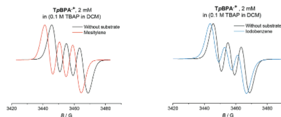
Fig. 10 EPR spectra of \text{TpBPA}^+ with reactive mesitylene (left, 350 eq.) and unreactive iodobenzene (right, 350 eq.).
