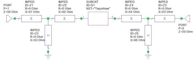
FIGURE 7. Adopted structure of the input and output matching sections.
