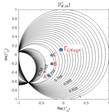
FIGURE 9. Level curves of the input Kurokawa reflection coefficient magnitude |\Gamma'_{K,in}| in the source reflection coefficient plane \Gamma'_G ; the star markers denote cases A, B and C. All points lay in a region where |\Gamma'_{in}| < 0.752 , the minimum being 0.74, see Table 1. \Gamma_{GNopt} is the optimum noise source reflection coefficient. Notice that the range of \Gamma'_G values for which the level curves are shown is limited to unity.
