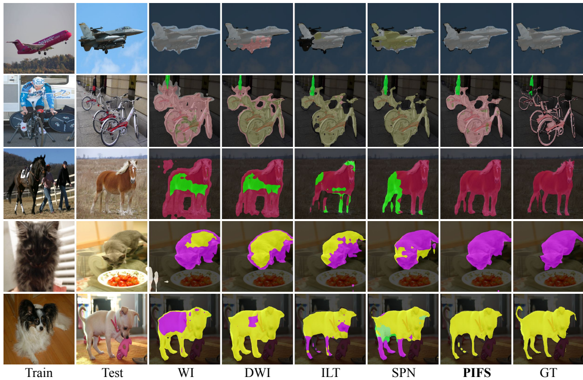
Fig. 4.3 Qualitative results on the VOC-SS 1-shot setting.
