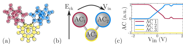
Fig. 3. MoSQuiTo methodology: (a) schematic representation of the atomic charges of a molecule, di-ferrocenyl carborane is used as an example, (b) definition of the principal electrical figures of merit that describe the electrostatic behavior of a molecule, (c) VACT graph for the bis-ferrocene molecule when the clock field equals 2 \text{ V/nm} .
