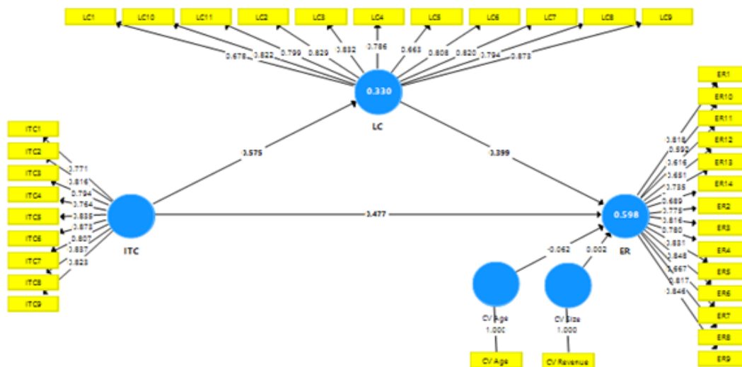
Figure 1: Path model
