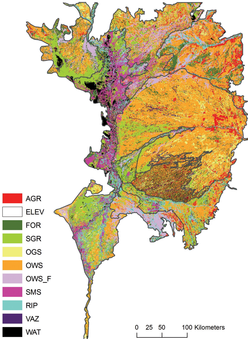
Figure 3 - Habitat classification for the Pantanal. AGR (agriculture), ELEV (Elevated areas not subject to inundation), FOR (Forest), SGR (Swampy grassland), OGS (Open grass savanna), OWS (Open woody savanna), OWS_F (Open woody savanna – flooded), SMS (Swampy mixed savannah), RIP (Riparian forest), VAZ (Vazante), Water (Open water not covered by vegetation canopies)
