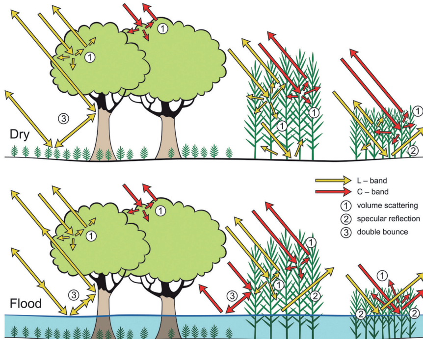
Figure 1 - C and L-band SAR interactions in tropical wetlands
