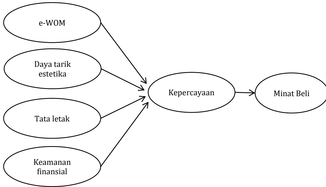
Gambar 2. Model Penelitian
