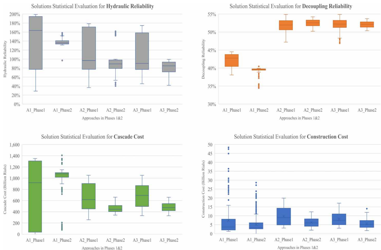
Figure 6 | Descriptive statistics of Pareto fronts in Figure 5 through box plots.
