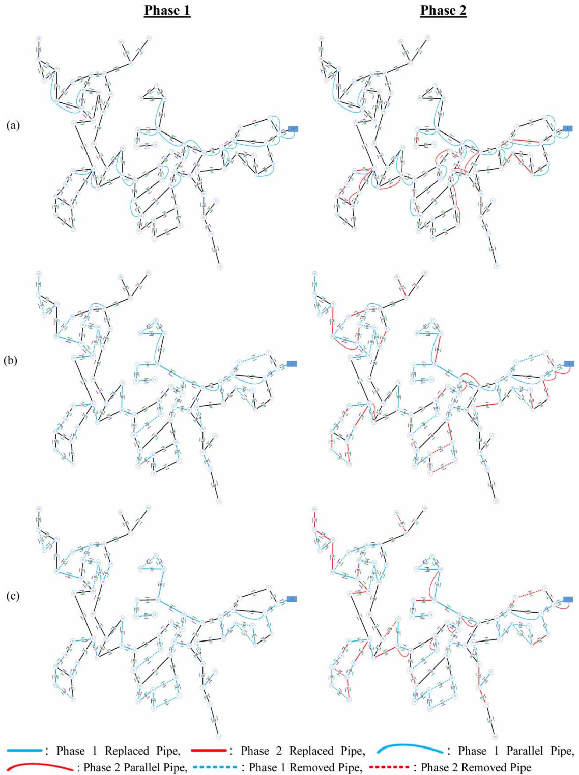
Figure 7 | Manifestation of constructed intervention plans in Phases 1 and 2 offered in Table 4, (a) A1, (b) A2 and (c) A3.
