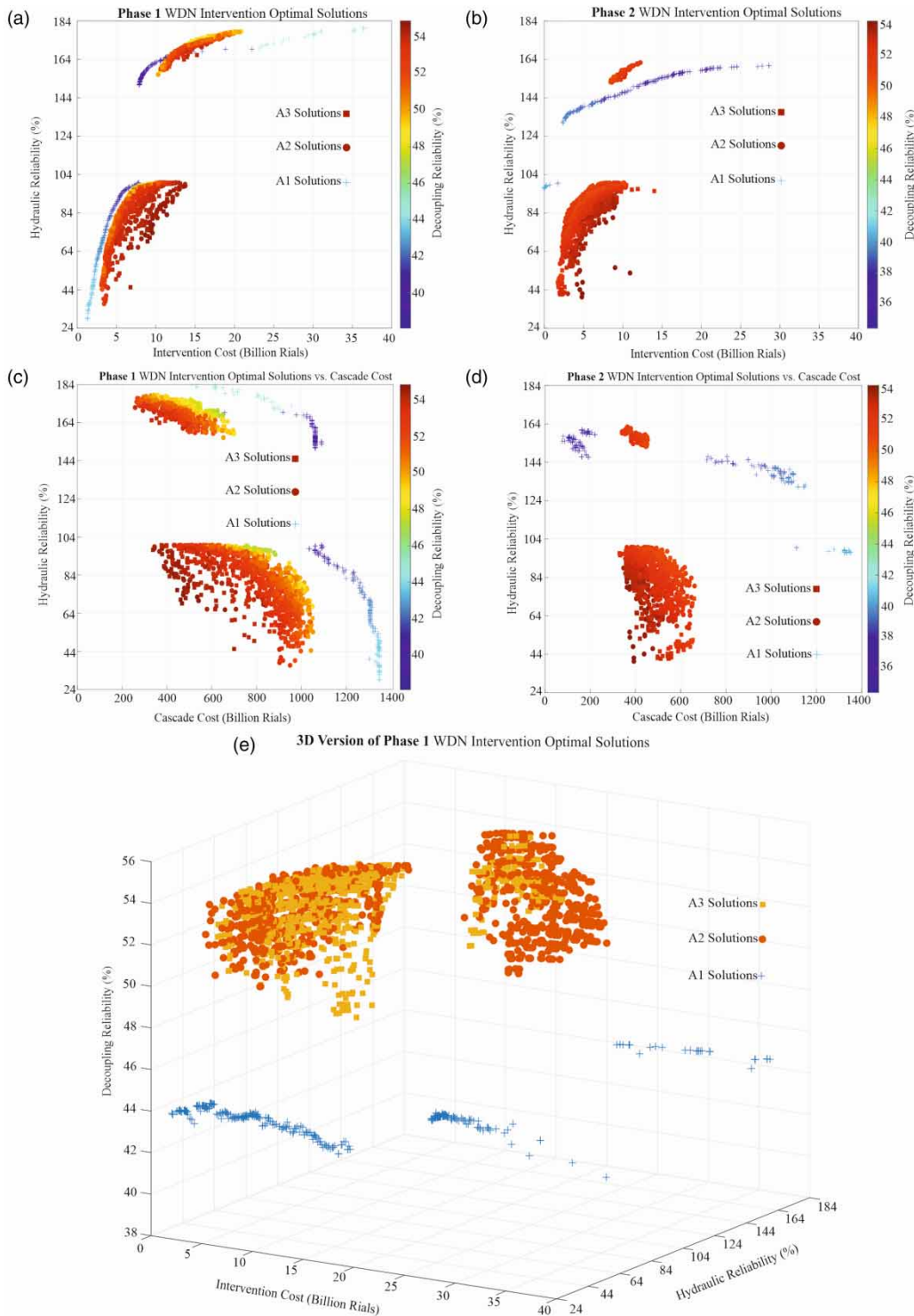
Figure 5 | Pareto fronts solutions from different approaches. The solutions with hydraulic reliability lower than 100% are in the weak set, while the ones with hydraulic reliability over than 100% are in the robust set (the gap between distinct regions means jumping from weak to robust (resilient) condition).
