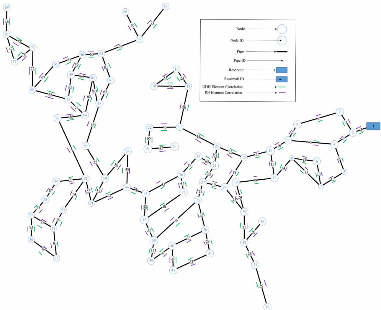
Figure 4 | Baghmalek WDN and correlation with adjacent networks' elements in year 0.
