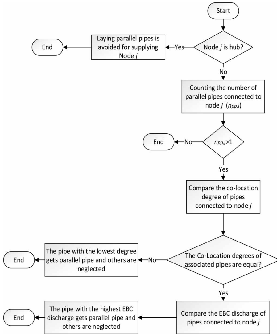
Figure 3 | The decision-making algorithm of laying parallel pipes in A3 for intervention planning of WDN.
