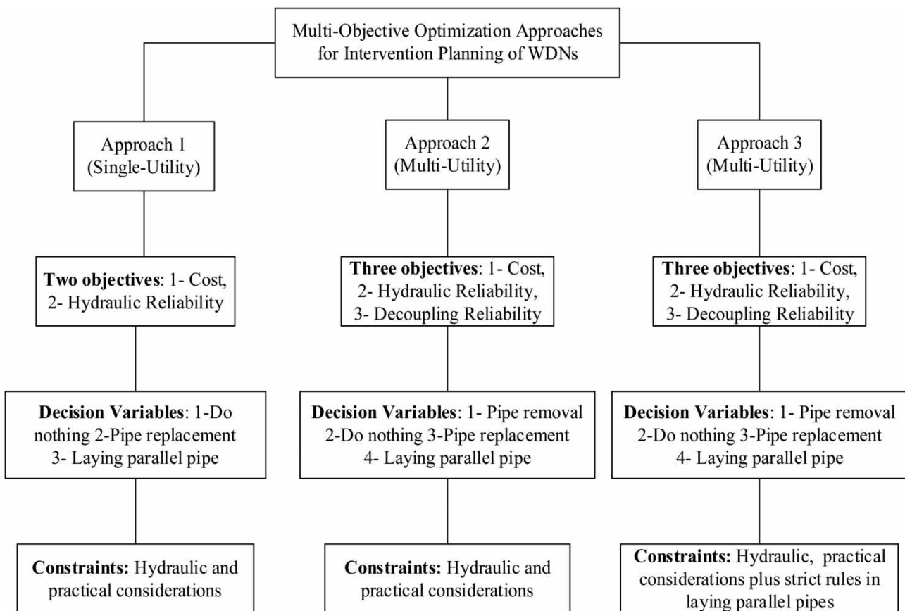
Figure 1 | Single and multi-utility approaches for intervention planning of WDNs.
